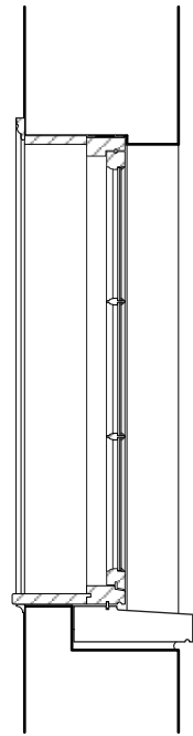
Section 1:20
