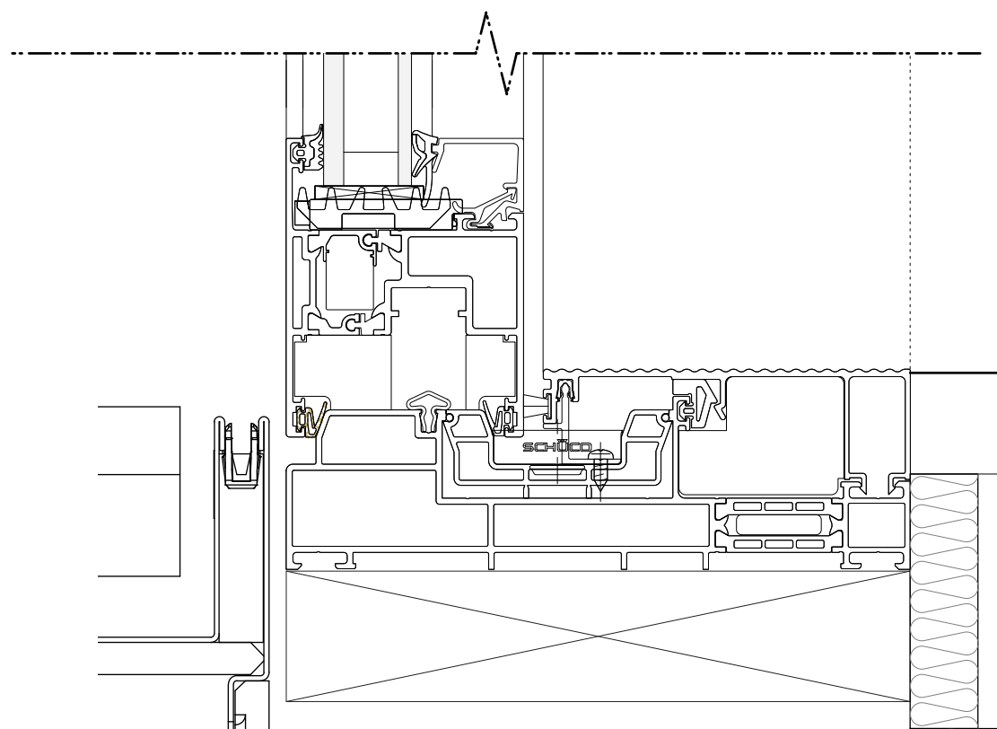
Section Detail through Bottom of Sliding Vent 1:2
