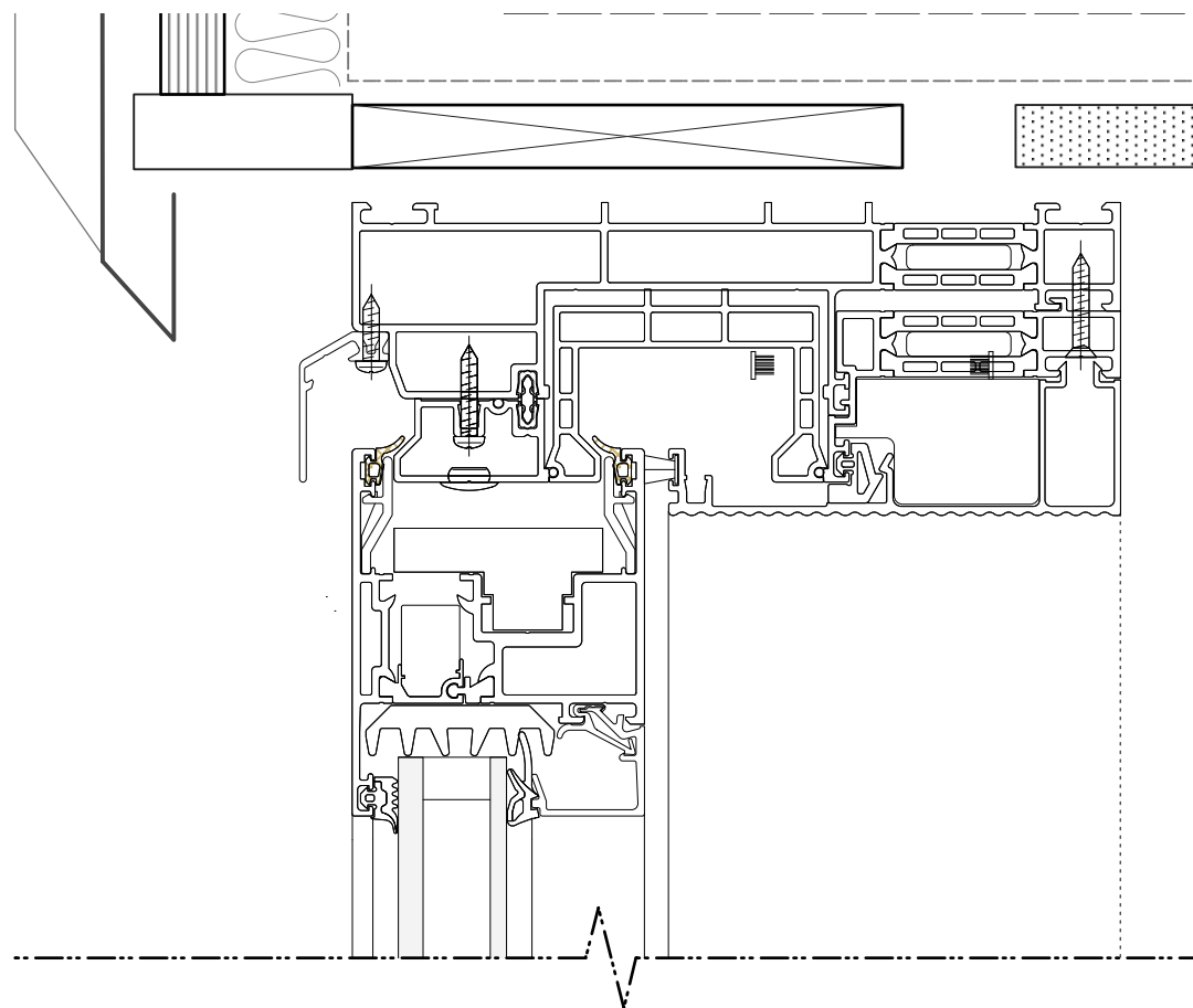
Section Detail through Head of Sliding Vent 1:2
