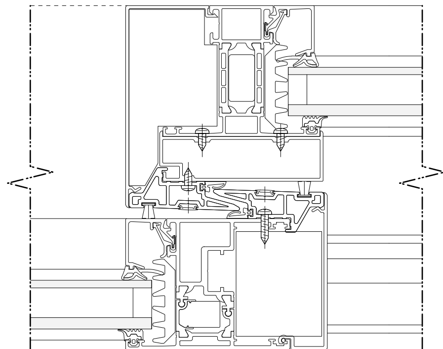
Plan Detail through Sliding Vent and Fixed Light 1:2
