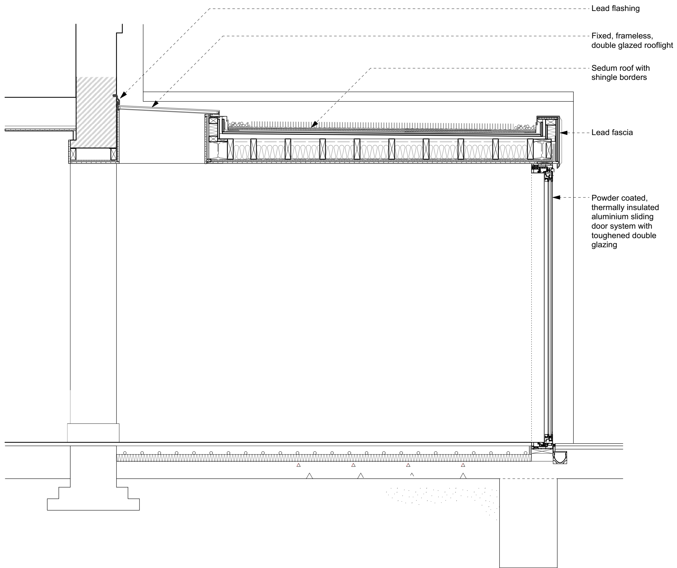
Proposed DETAILS _ Conservatory Extension_ Section I
