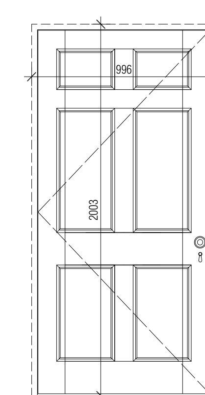
Type 09 4 Panel painted door (Panel mould 1) Master Bedroom
