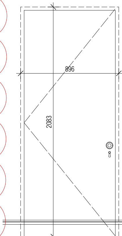
Type 19 Jib Door to Rear Landing DF15-1 - Type 11 facing the other side
