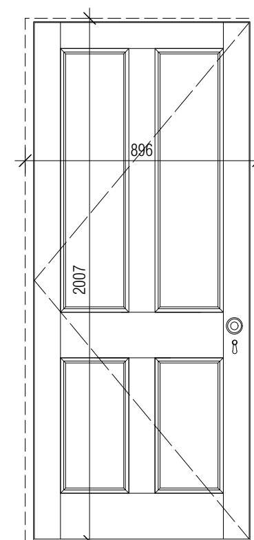
Type 10 4 Panel Painted Door (Panel mould 2) Lower Ground Floor
