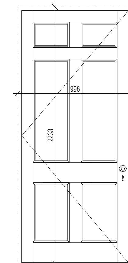
Type 16 Primary 6 Panel (Panel mould 1) Painted door
