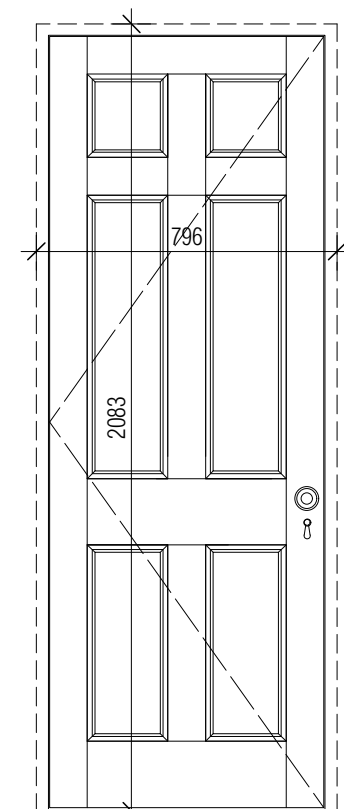
Type 12 6 Panel Painted Door (Panel mould 2)
