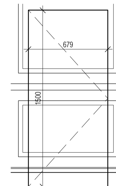
Type 13 Cub'd jib door to match panel/mouldings Rear vestibule
