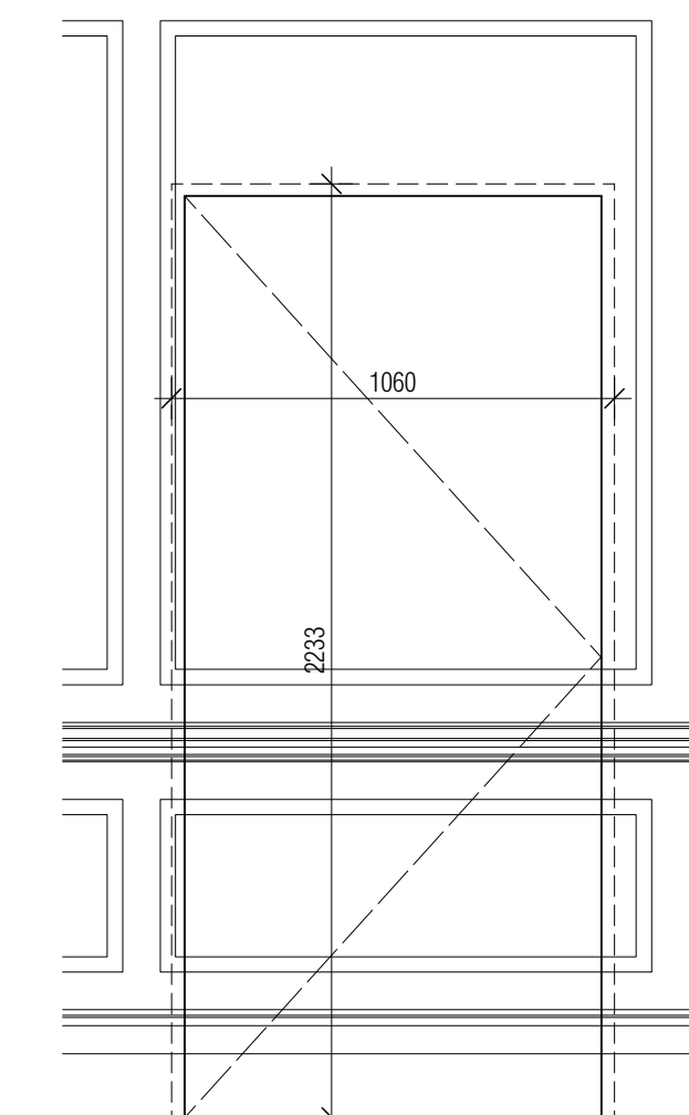
Type 18 Jib Door to Dining Hall DG13-1 - Type 6 facing the other side
