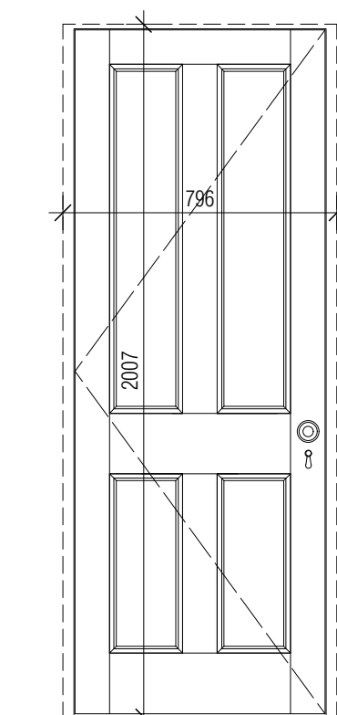
Type 17 4 Panel Painted Door (Panel mould 2) Lower Ground Floor
