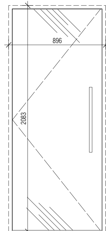
Type 04 Glass door Shower rooms
