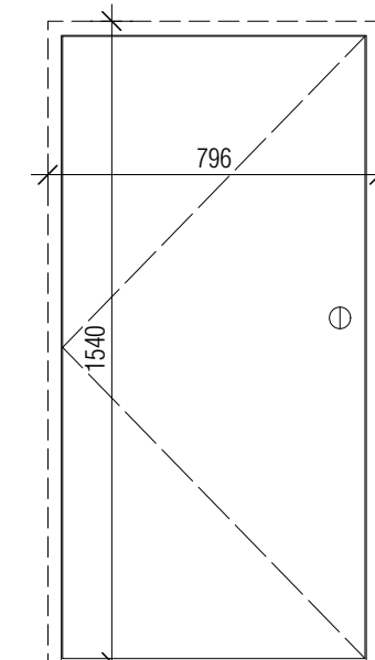
Type 14 Cub'd jib door Understairs cub'd
