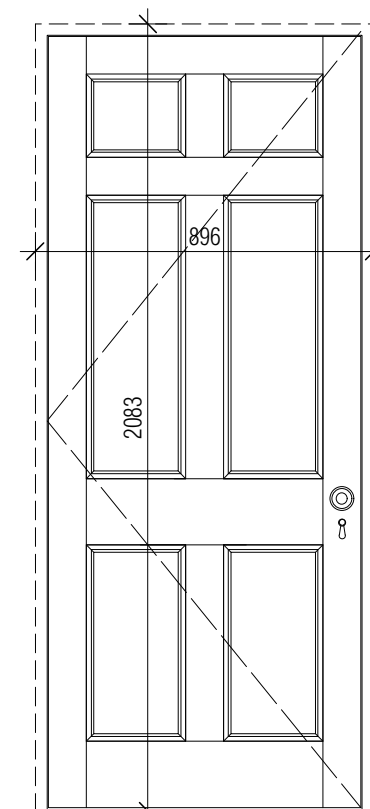
Type 11 6 Panel Painted Door (Panel mould 2)
