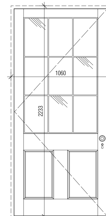
Type 15 Part Glazed door (Panel mould 1) Panel Door
