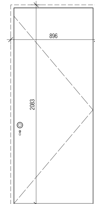
Type 03 Painted Plywood faced door
