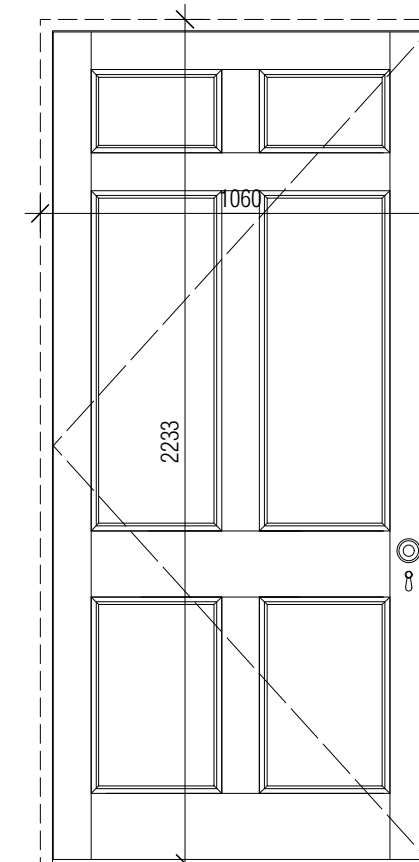
Type 06 Primary 6 Panel painted door (Panel mould 1)
