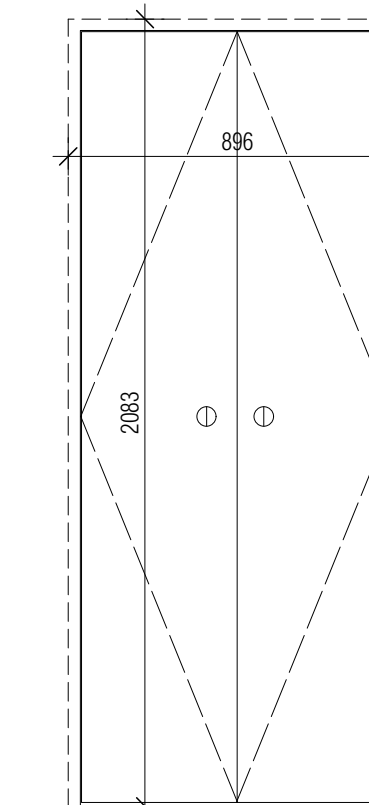
Type 08 Lobby cup'd door Panelled jib door tbc
