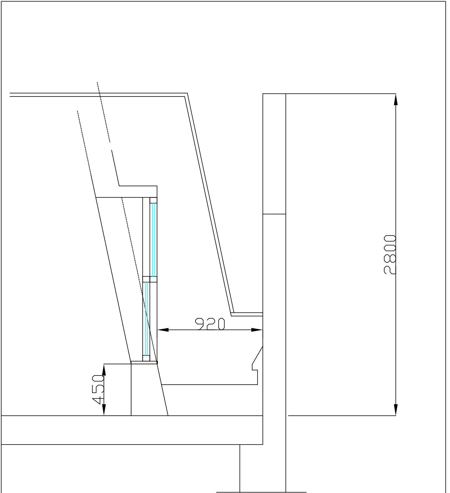
277 Gray's Inn Road Section thro' parapet
