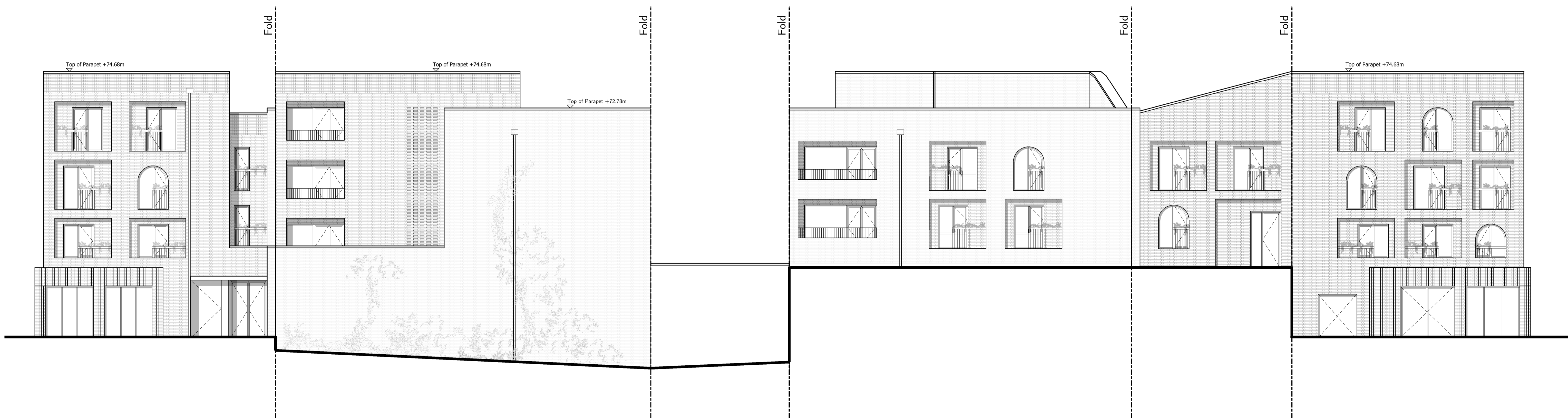
O Building B2 ELEVATION
