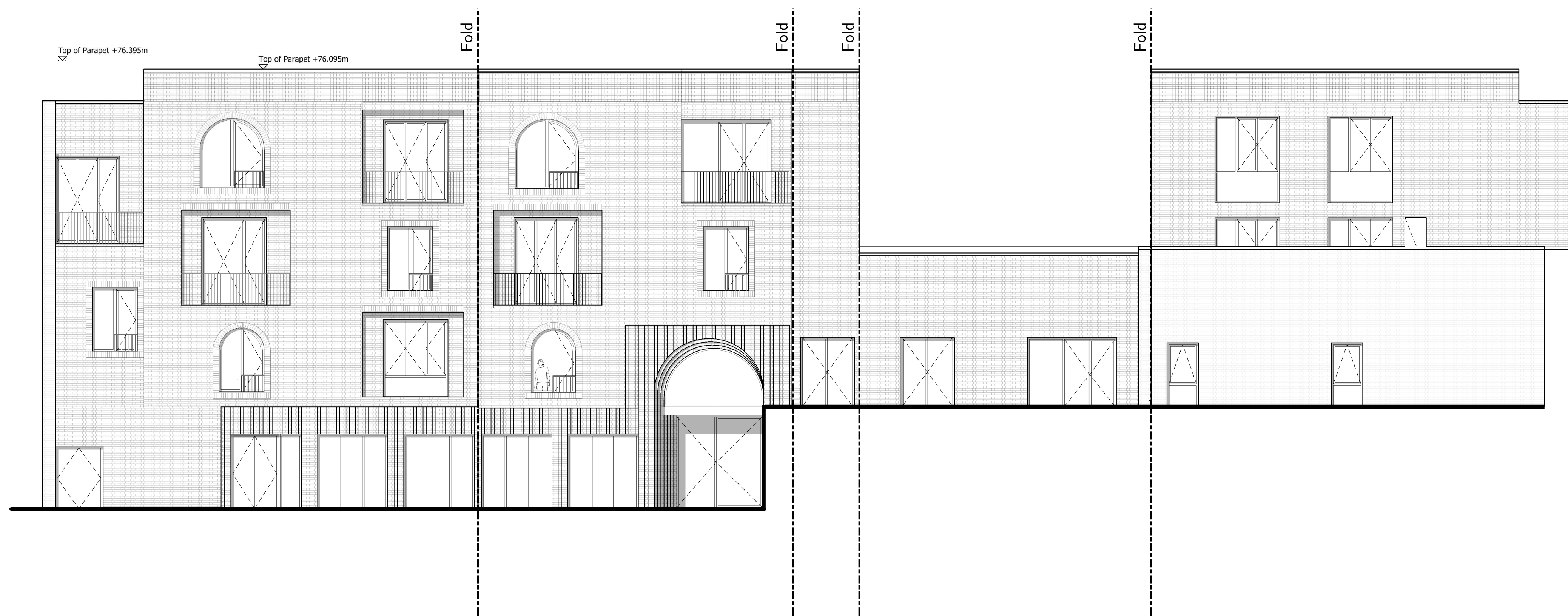
K Building B1 ELEVATION
