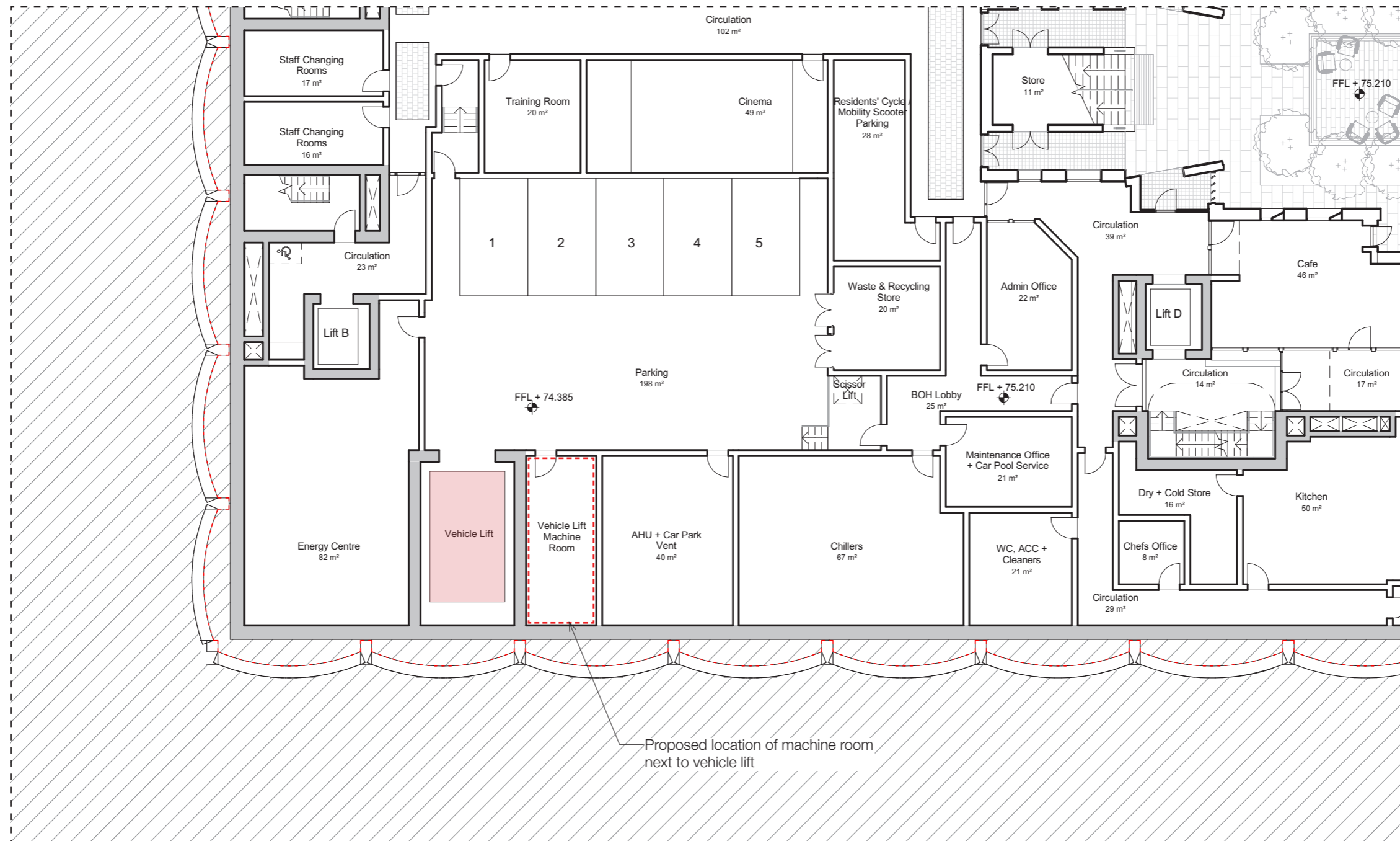
Level B1 Extract Plan - Vehicle Lift Machine Room Location Scale 1:200 @A3
