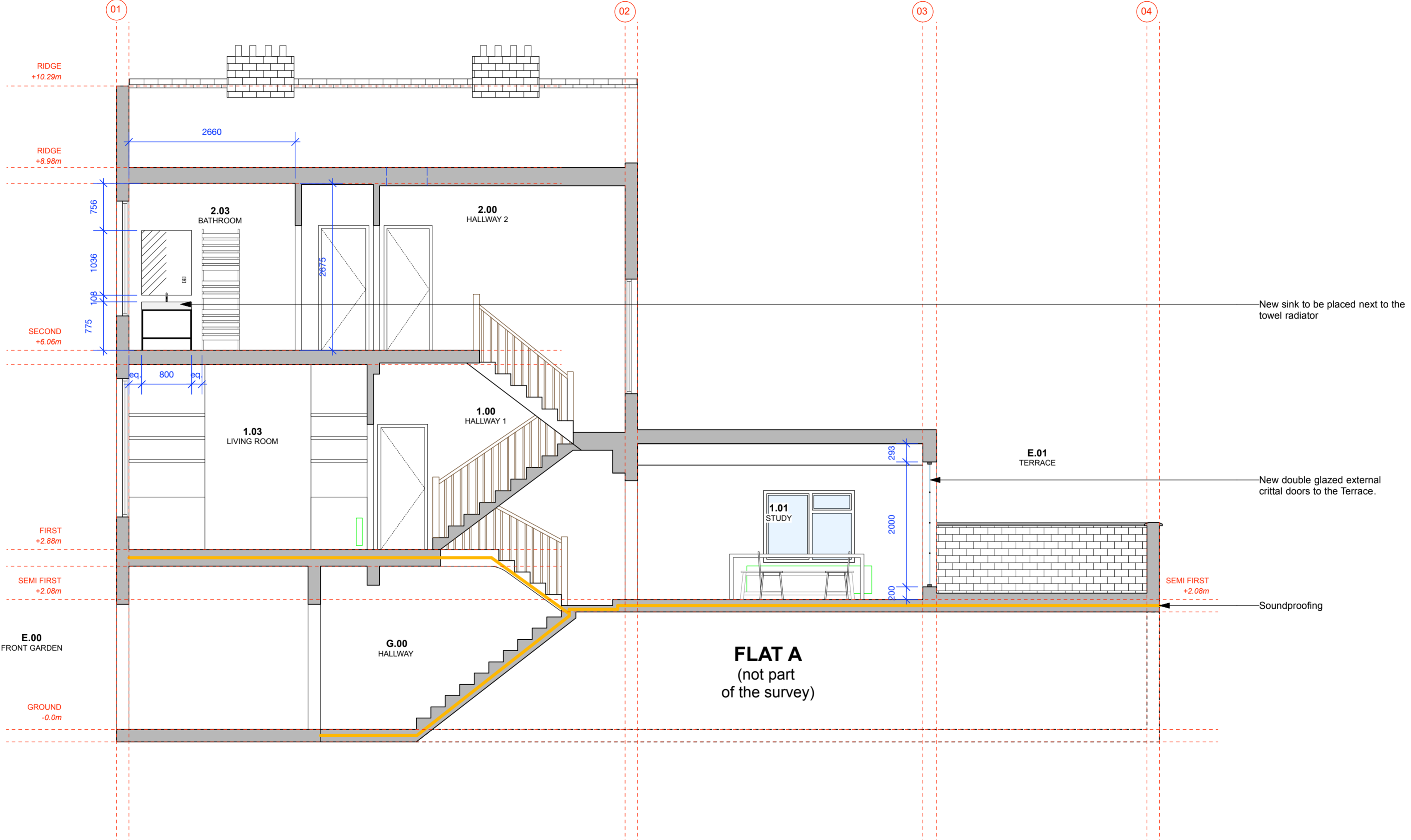
EXISTING SECTION A-A
