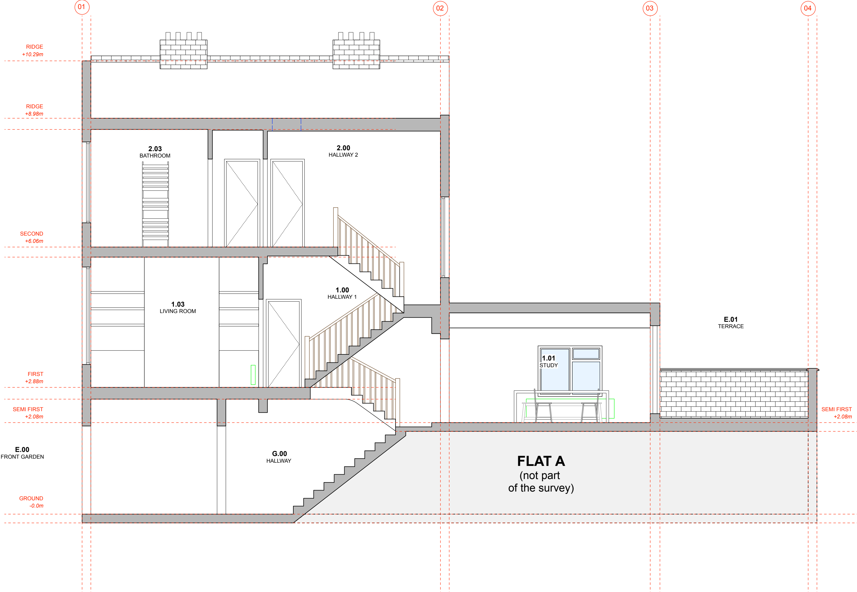
EXISTING SECTION A-A
