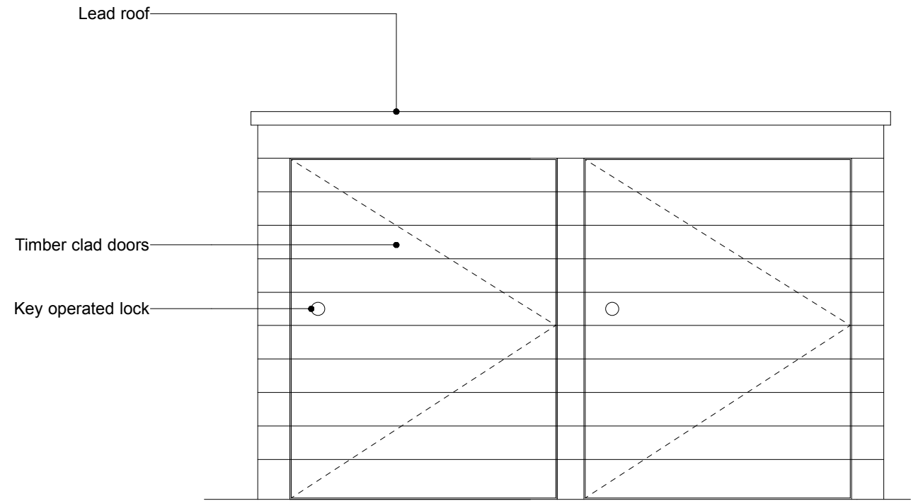
Front Elevation
