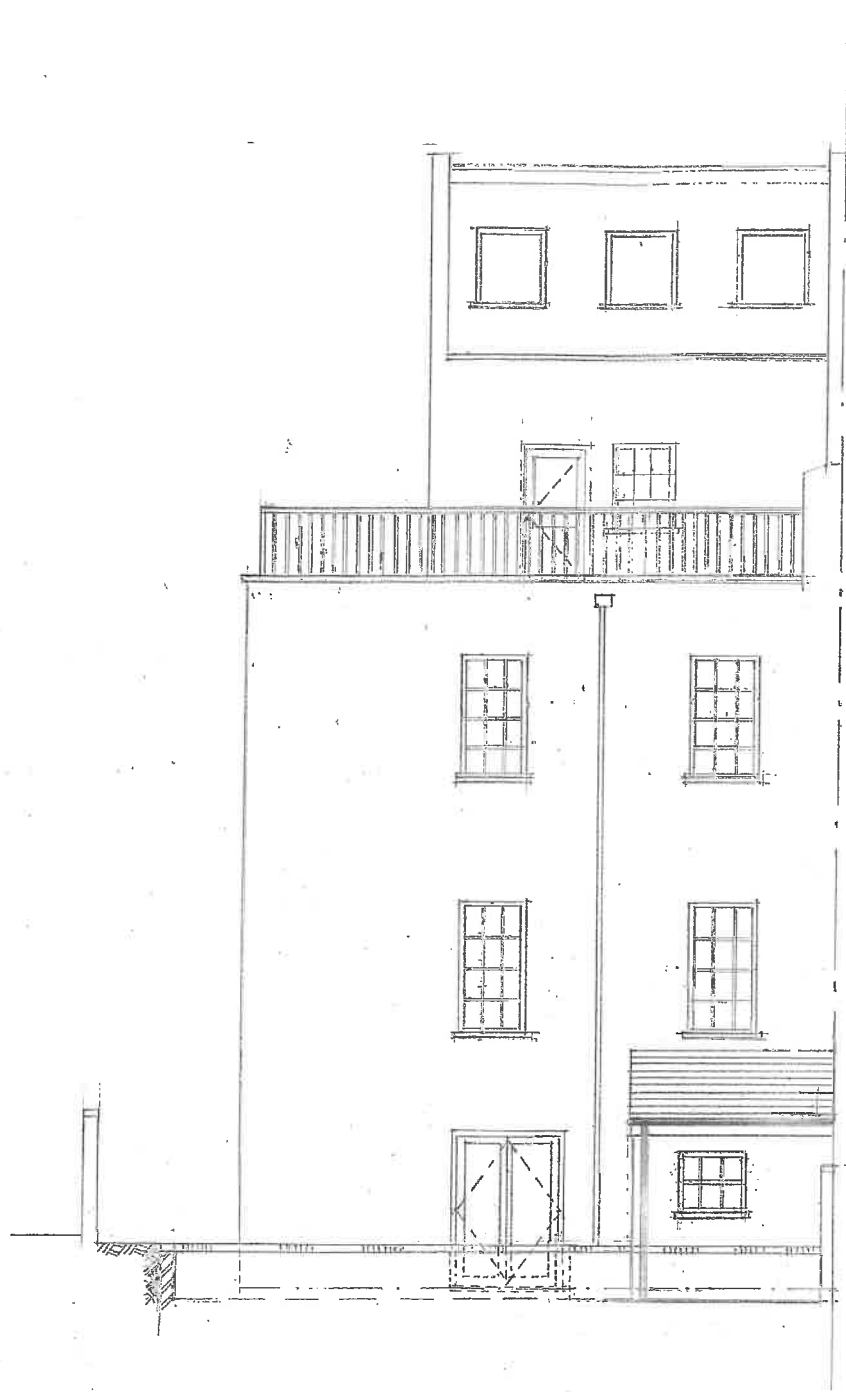
REAR ELEVATION AS EXISTING
