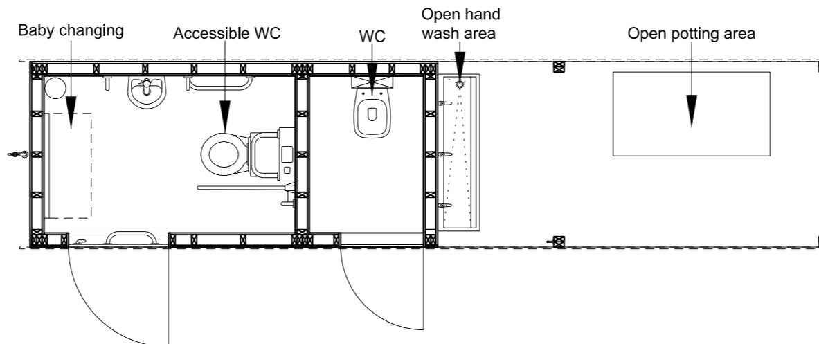
Ground Floor Plan (1:50)
