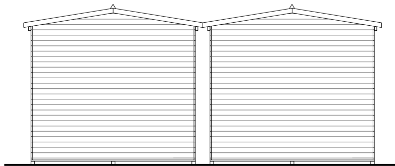
Elevation 3 (1:50)
