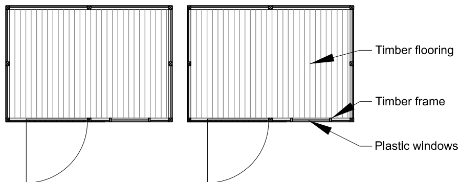
Ground Floor Plan (1:50)
