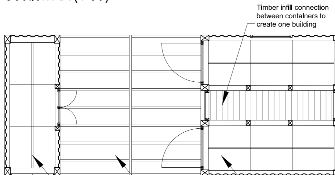
Section AA (1:50)
