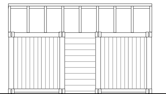
Elevation 3 (1:100)
