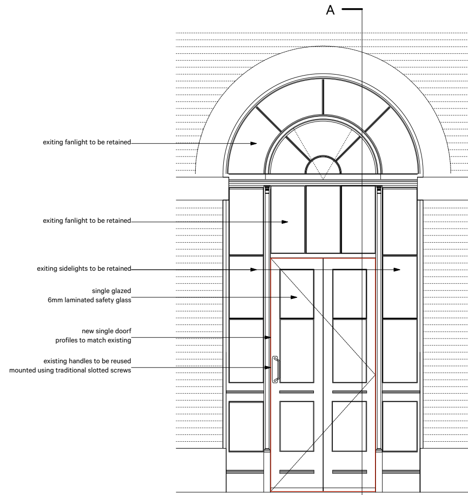
EXTERNAL ELEVATION
