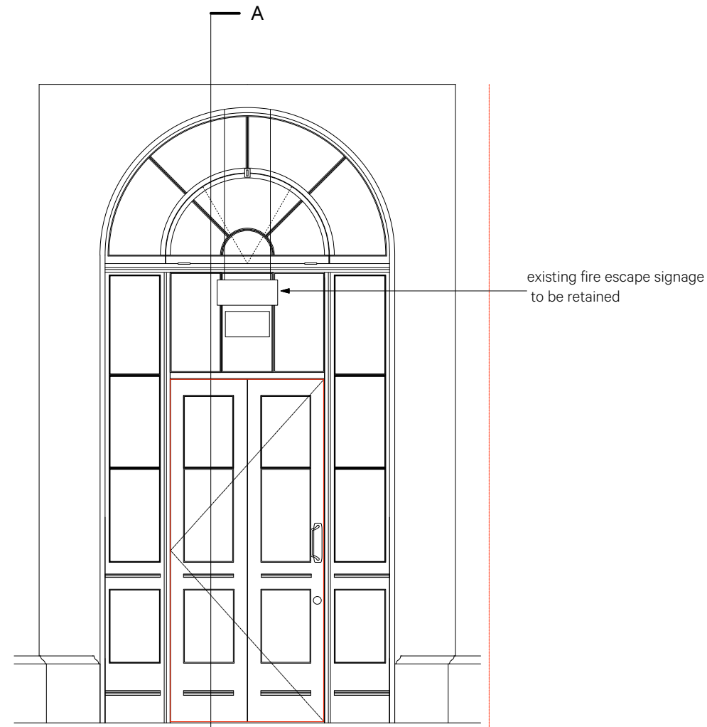
INTERNAL ELEVATION
