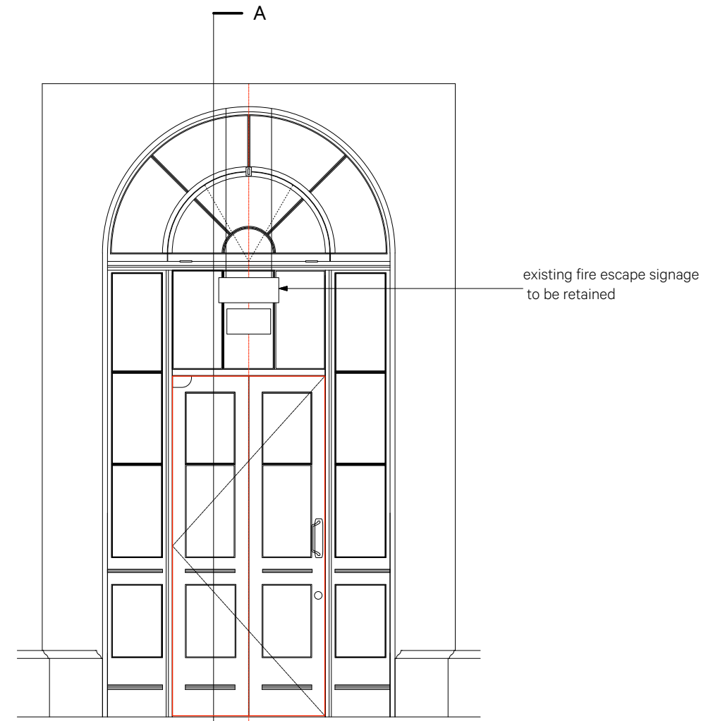
INTERNAL ELEVATION
