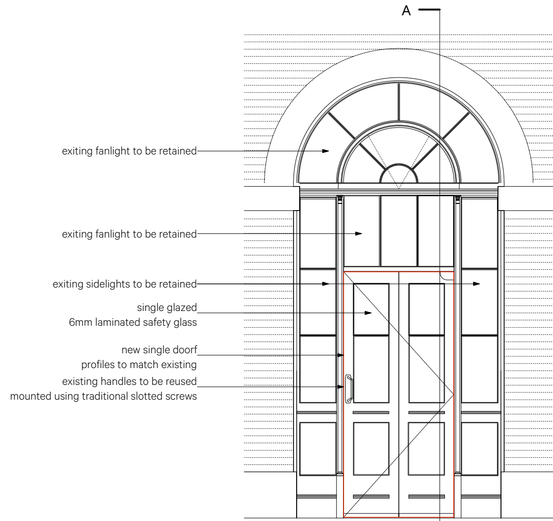
EXTERNAL ELEVATION
