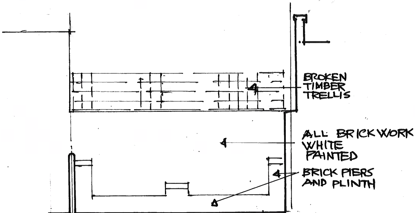
EXISTING REAR BOUNDARY WALL AND BROKEN TIMBER TRELLIS
