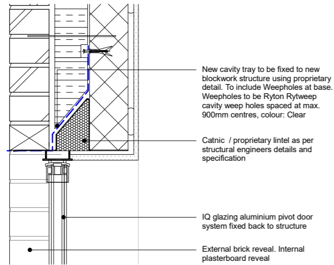
GF REAR ALUMINIUM PIVOT DOOR HEAD DETAIL Scale 1:10 @ A3
