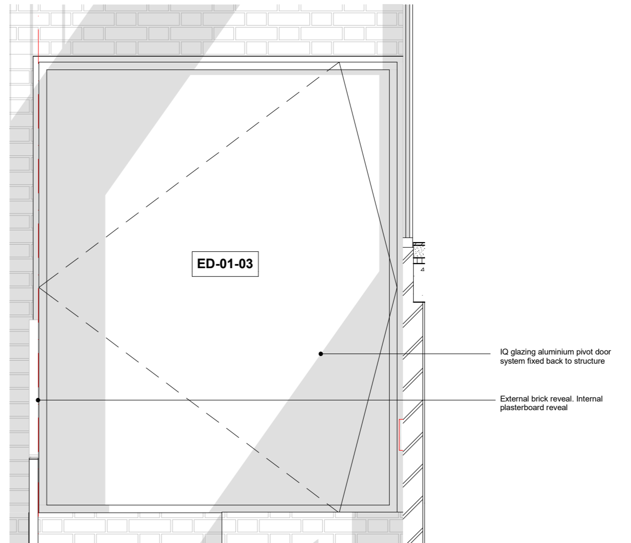
GF REAR ALUMINIUM PIVOT DOOR JAMB DETAIL Scale 1:10 @ A3
