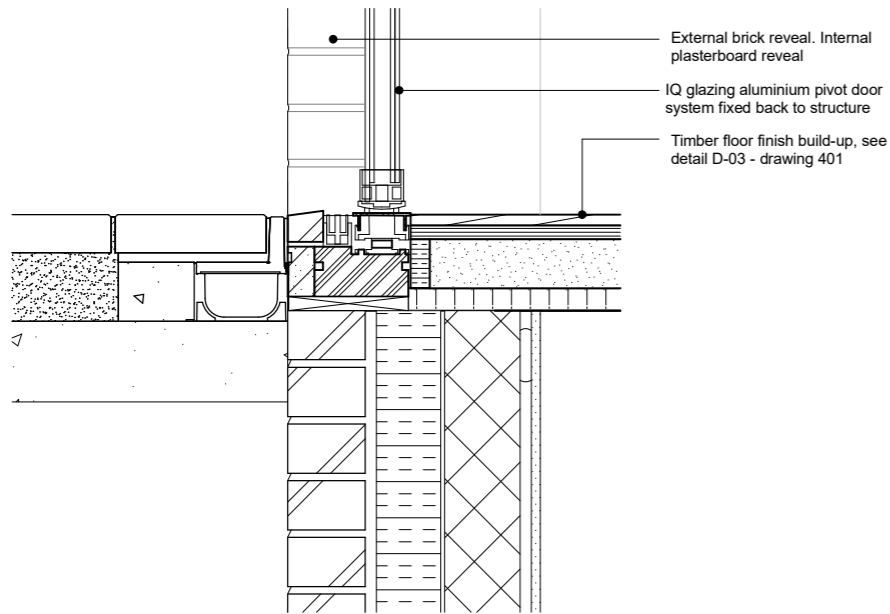
GF REAR ALUMINIUM PIVOT DOOR SILL DETAIL Scale 1:10 @ A3
