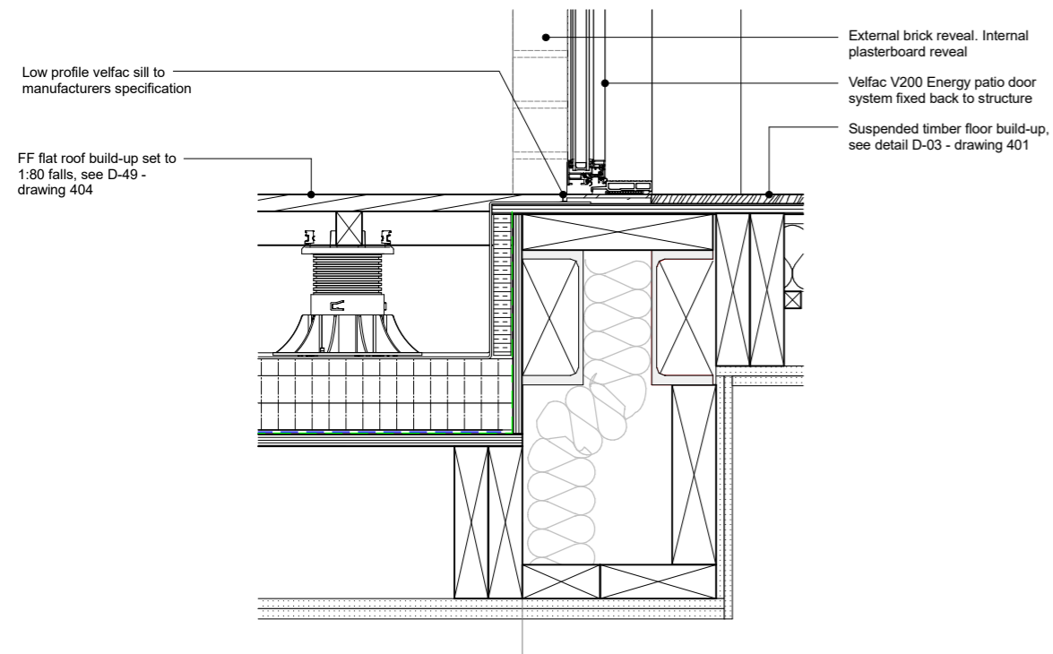
FF PATIO DOOR SILL DETAIL Scale 1:10 @ A3
