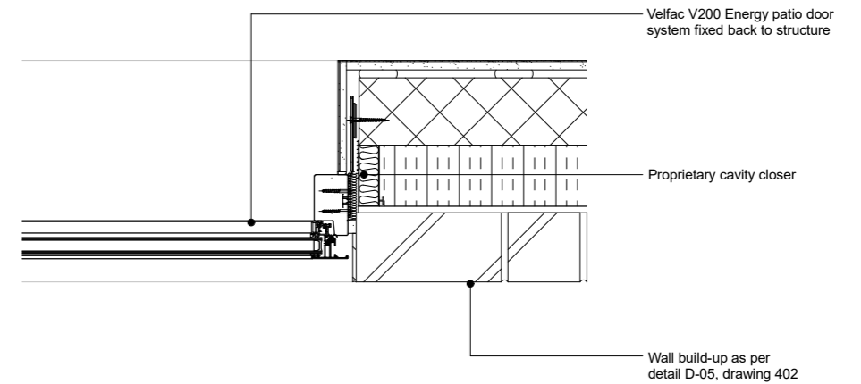
FF PATIO DOOR JAMB DETAIL Scale 1:10 @ A3
