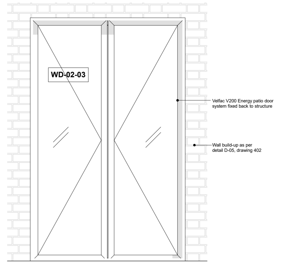
FF PATIO DOOR ELEVATION Scale 1:20 @ A3
