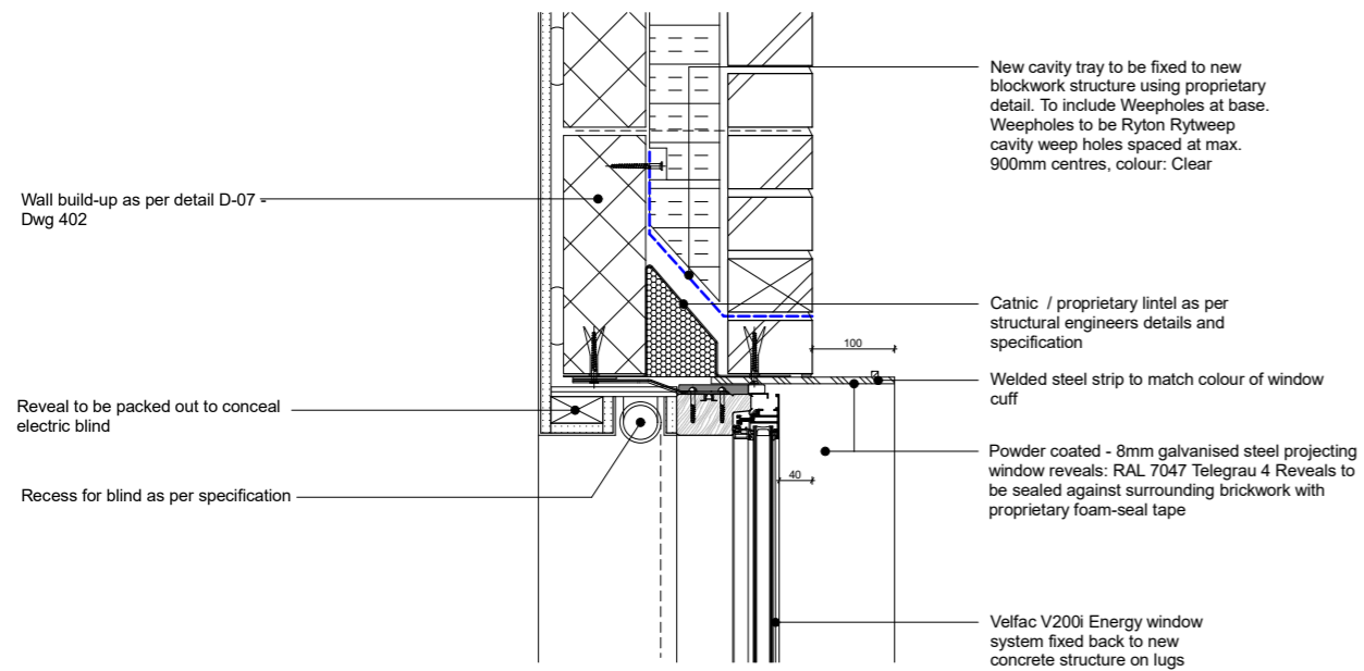
D-25 - TYPICAL WINDOW CUFF HEAD DETAIL SCALE: 1:10@A3
