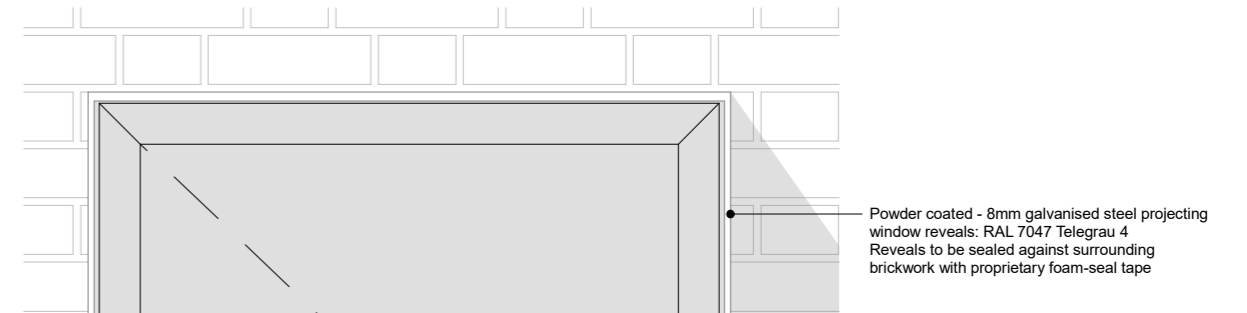
TYPICAL WINDOW HEAD ELEVATION SCALE 1:10 @A3
