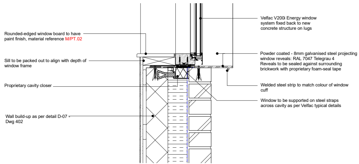
D-26 - TYPICAL WINDOW CUFF SILL DETAIL SCALE: 1:10@A3
