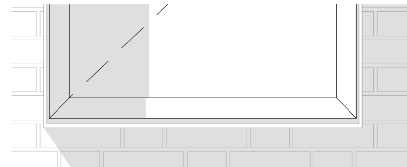
TYPICAL WINDOW SILL ELEVATION SCALE 1:10 @A3
