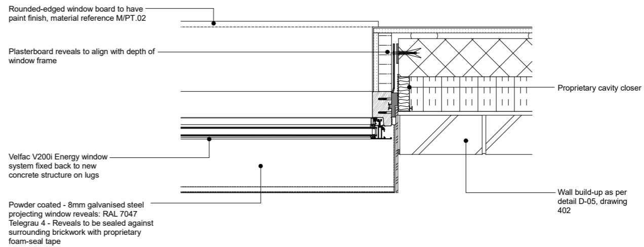
D-27 - TYPICAL WINDOW CUFF PLAN DETAIL SCALE: 1:10@A3
