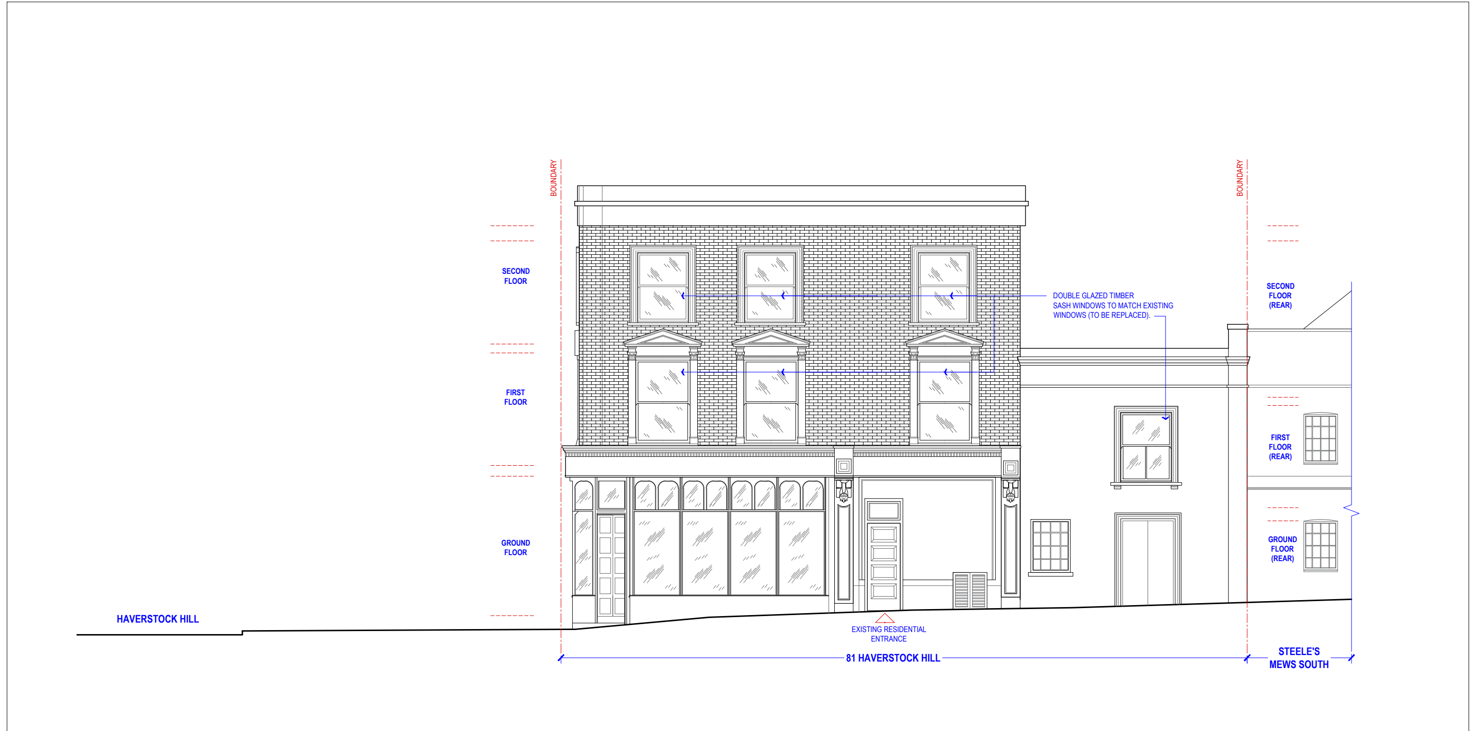
[01] PROPOSED SIDE ELEVATION
