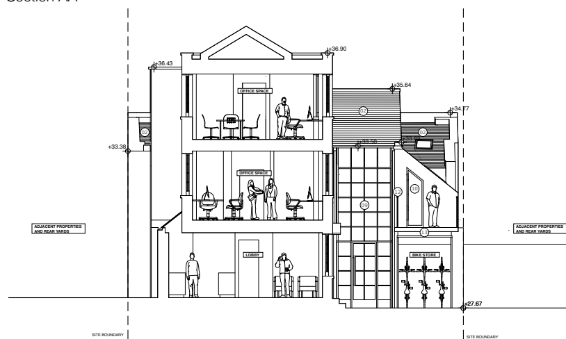
Elevation / Section BB
