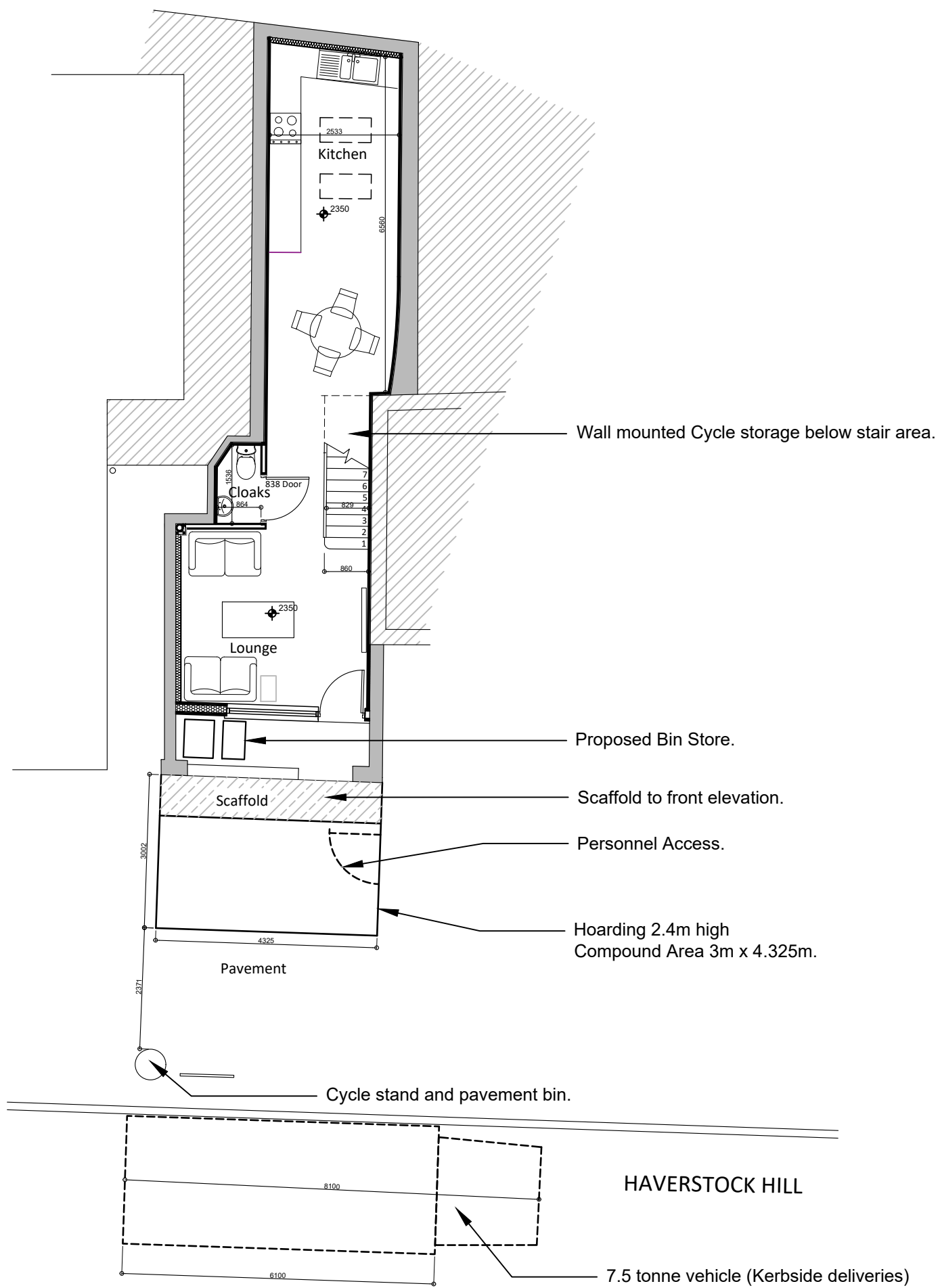
Ground Floor Plan - with Hoarding Detail to Front Scale 1:100
