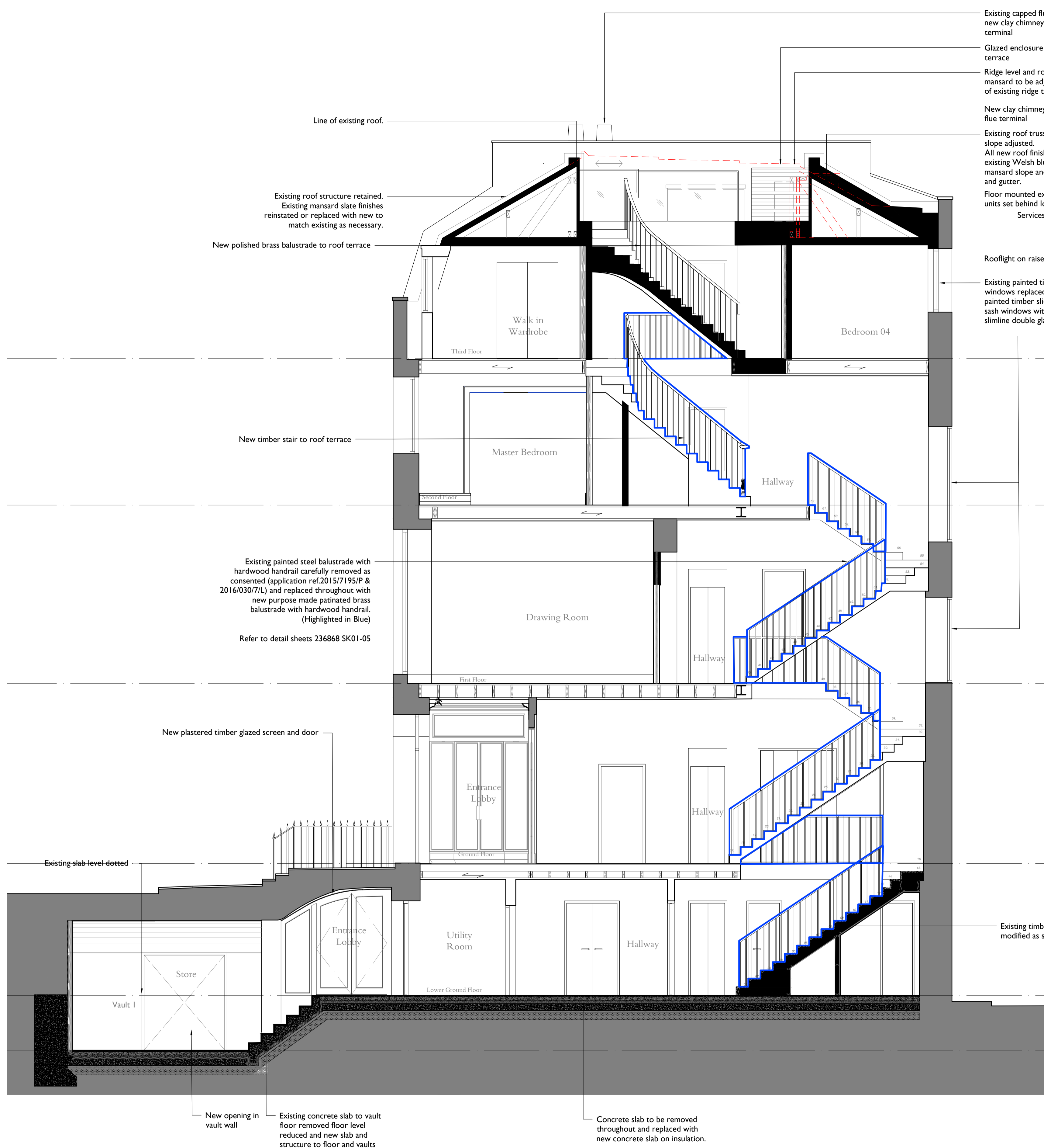
1 Proposed section AA 204 1:50@ A1 1:100@ A3
