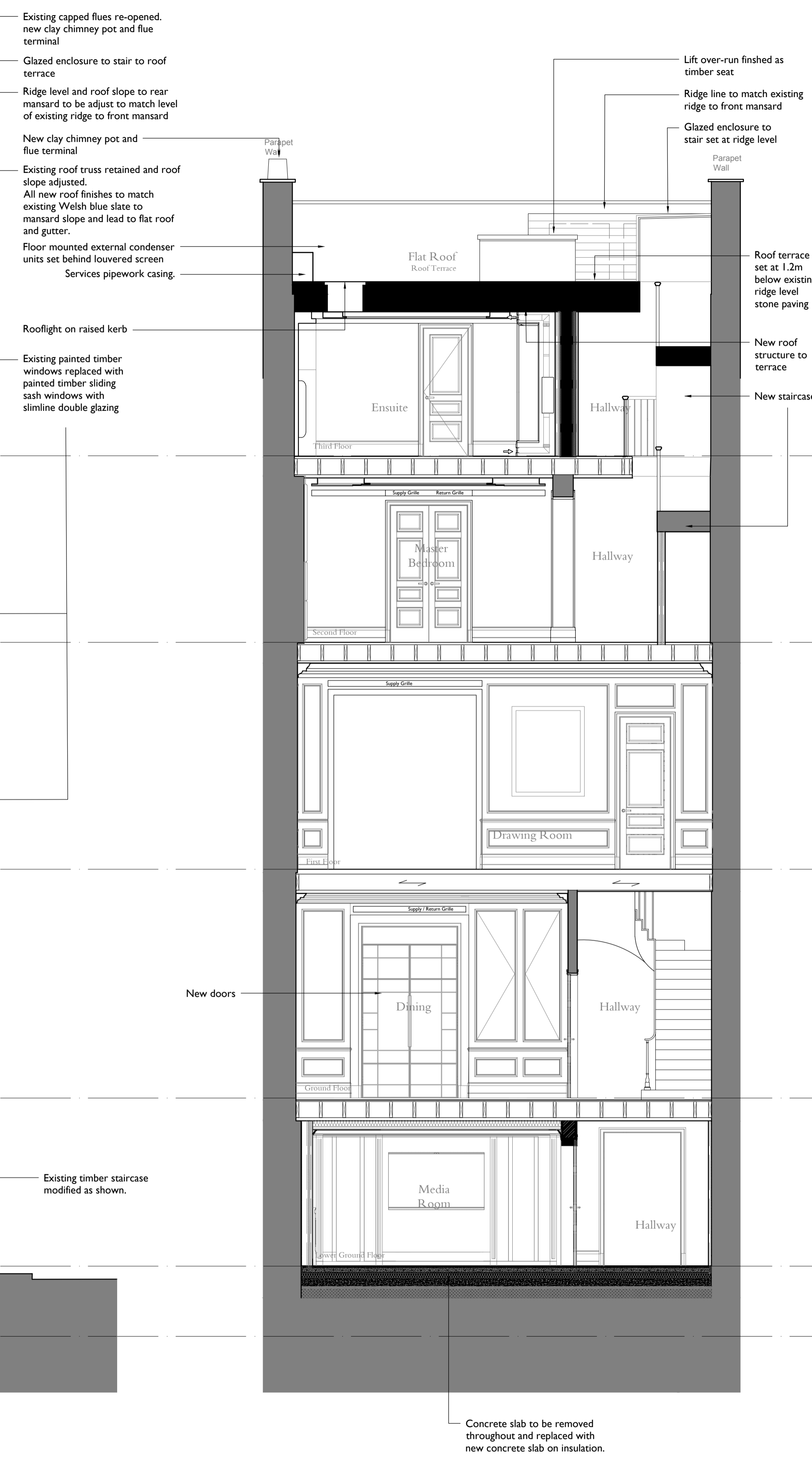
2 Proposed section BB 204 1:50@ A1 1:100@ A3
