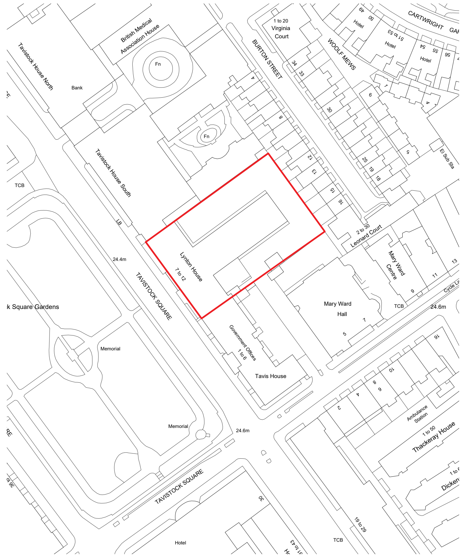
01 Site Location Plan 00.101 1:500@A1
