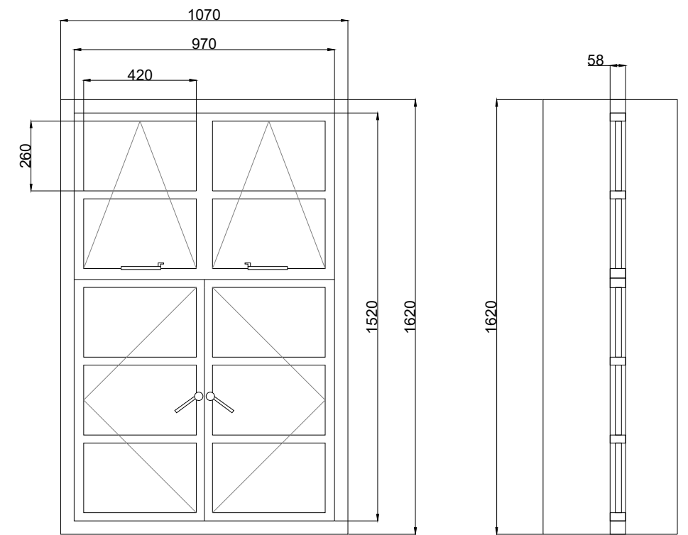
Existing Upper Floor Window Details
