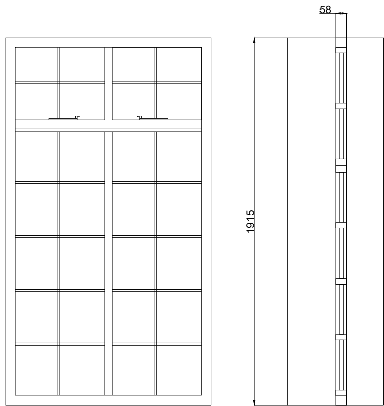
Existing GF Window Details
