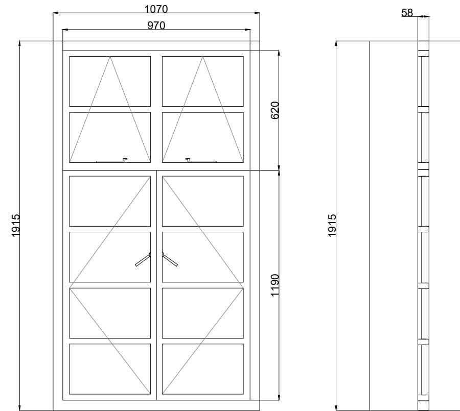
Existing FF Window Details
