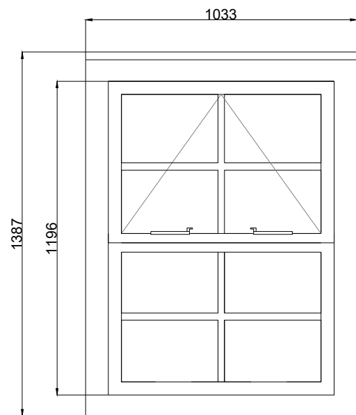
Type 1 Elevation
