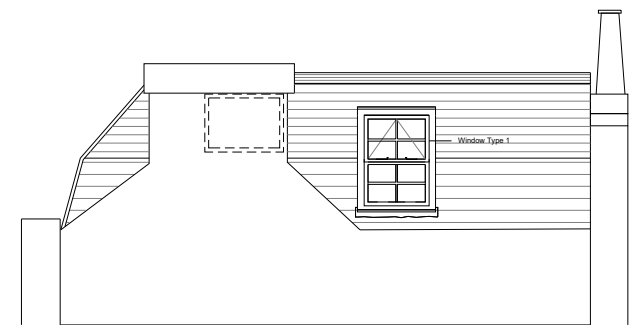
Rear Elevation
