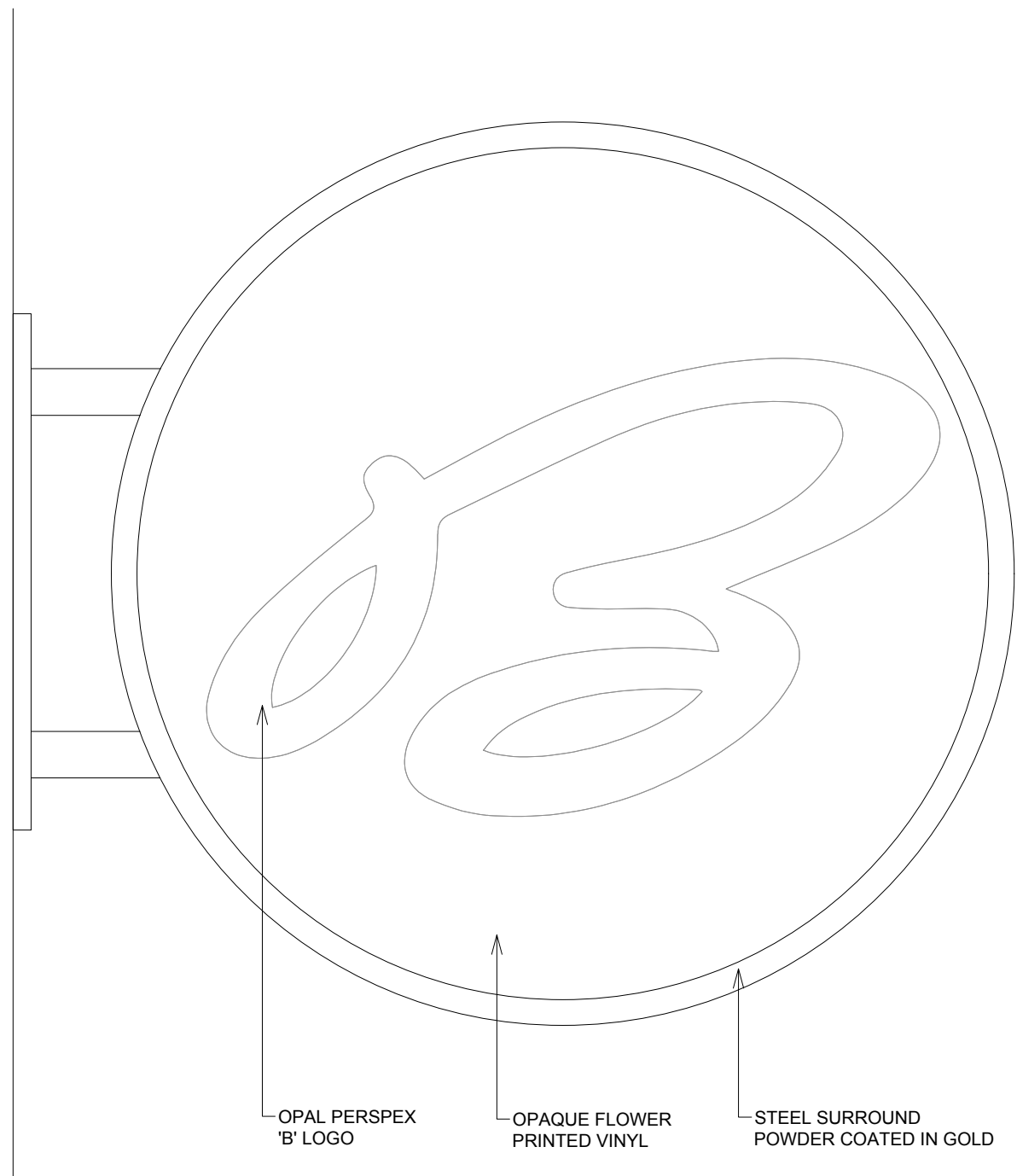
SIDE ELEVATION Scale 1:5
