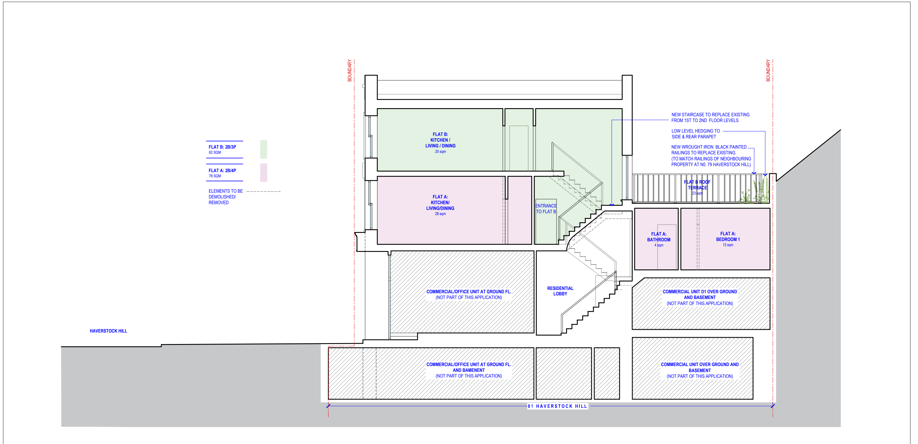
[01] PROPOSED SECTION AA'
