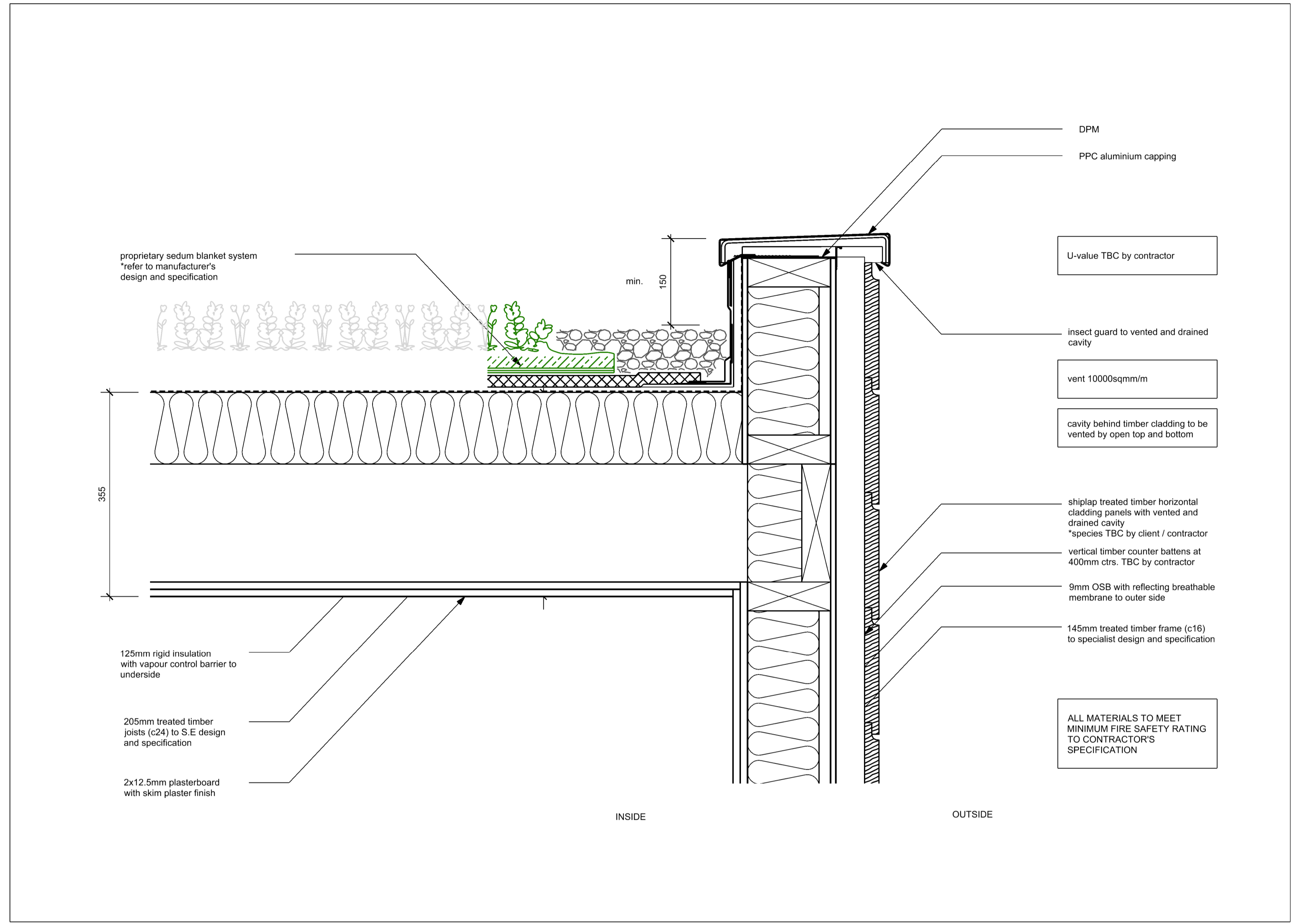
ROOF & PARAPET DETAIL
