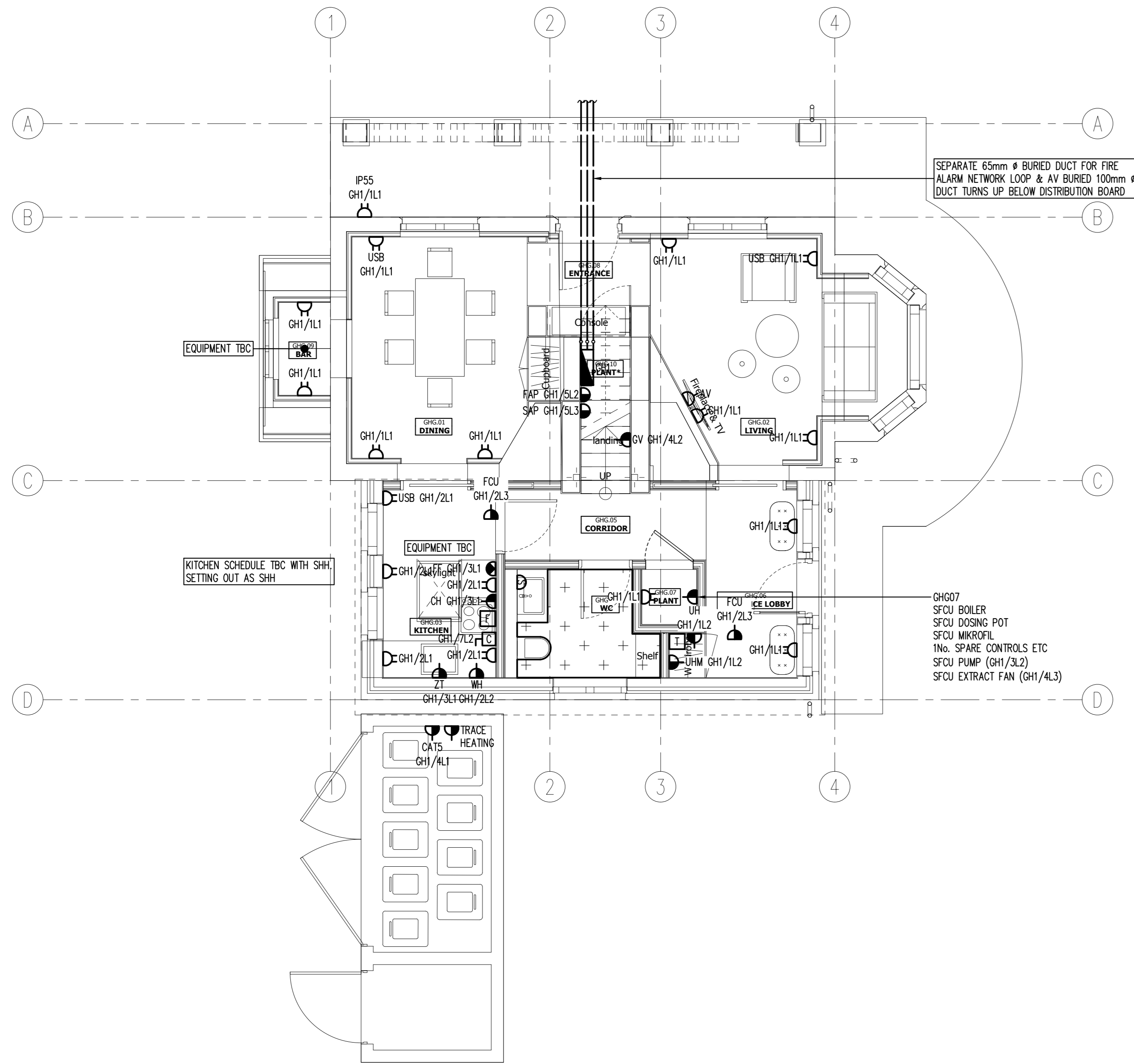
GATE HOUSE (GROUND FLOOR)
