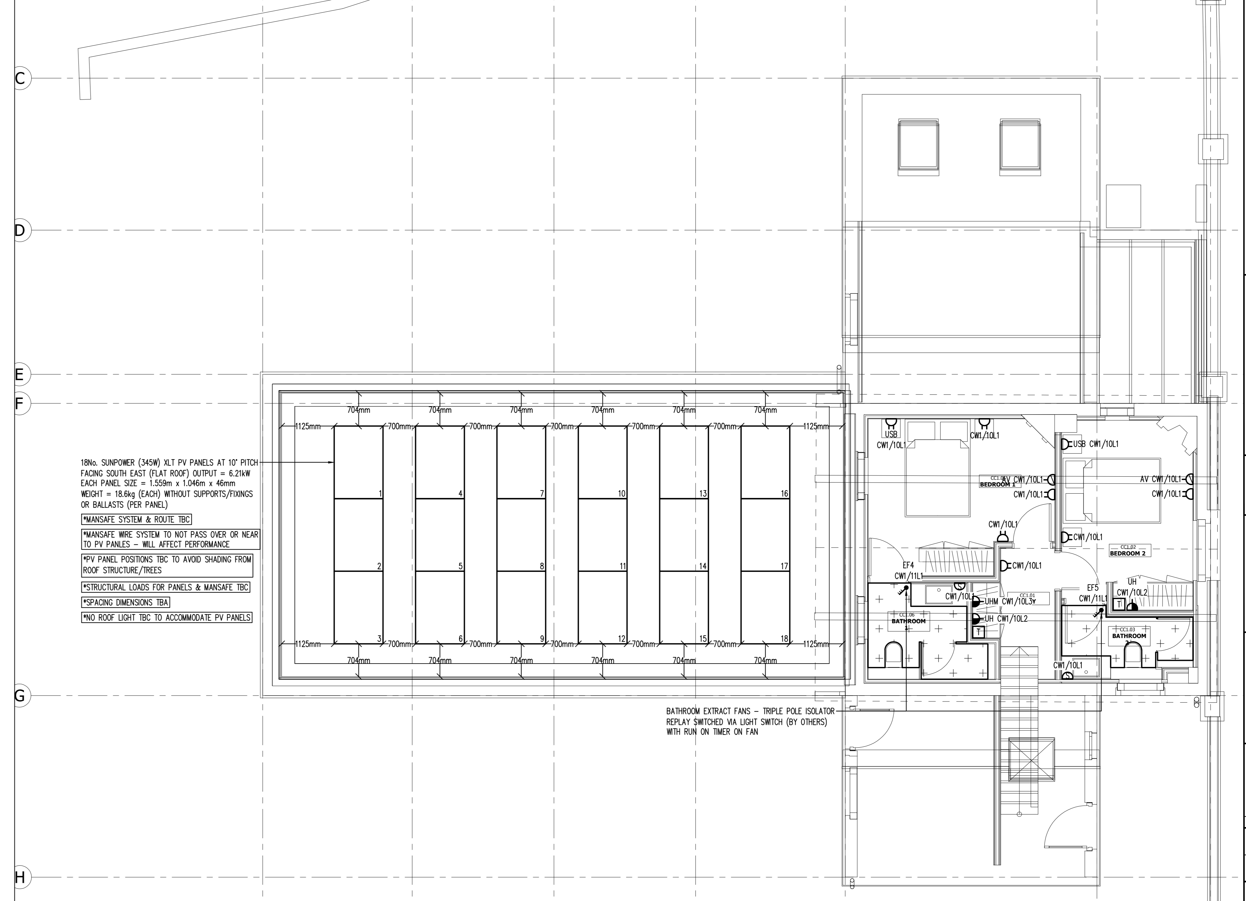
CAENWOOD COTTAGE (FIRST FLOOR)
