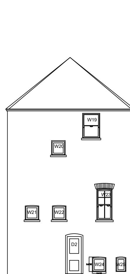
SIDE ELEVATION (Existing)
