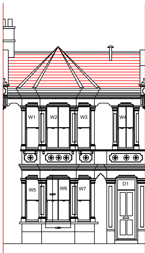
FRONT ELEVATION (Existing)
