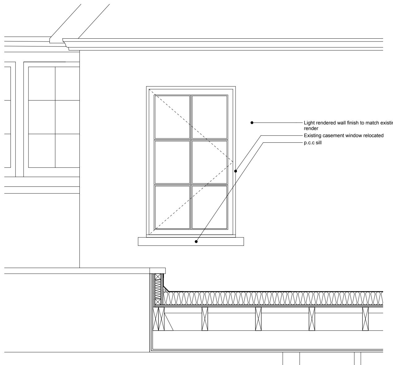
Proposed Window Elevation
