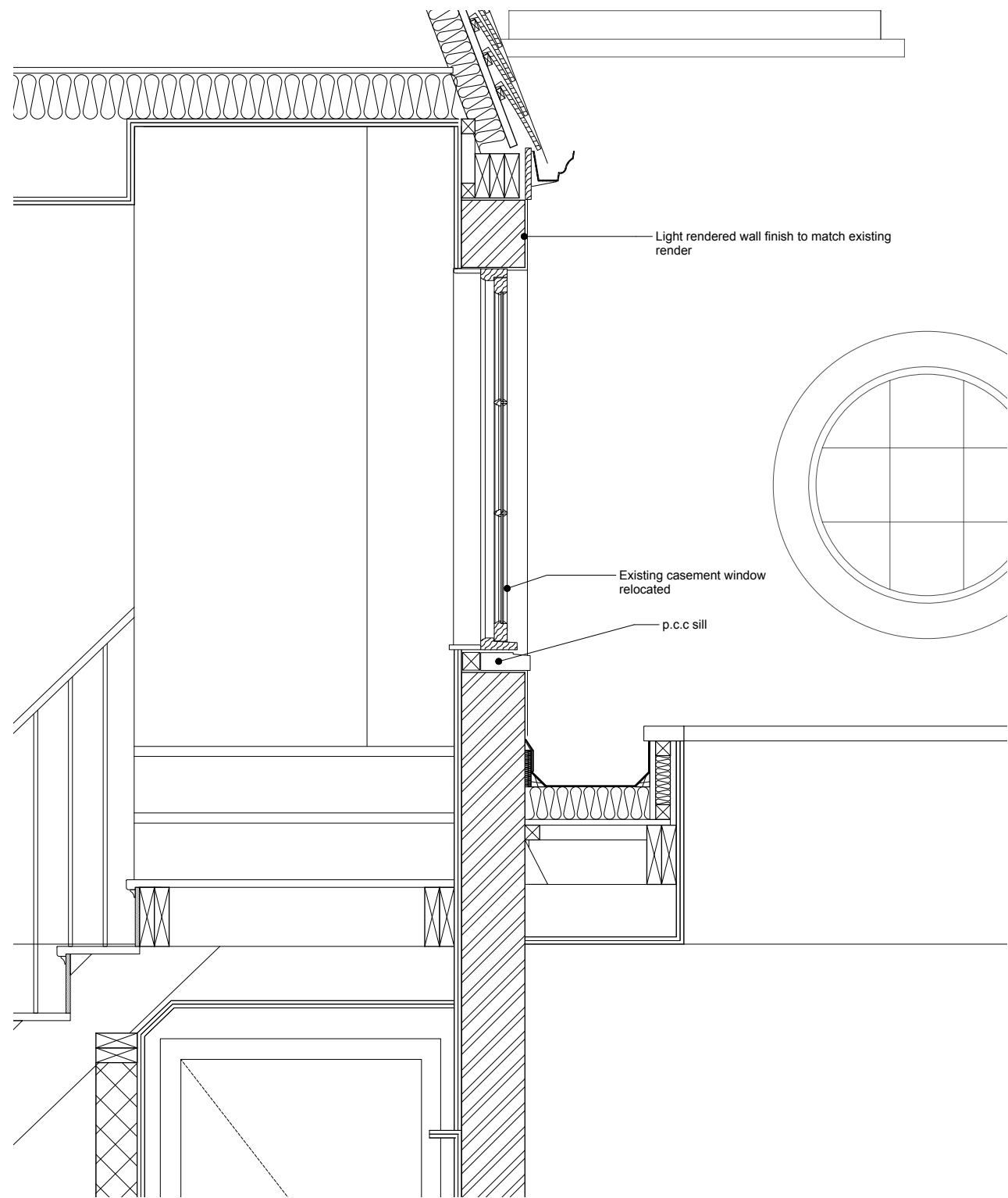
Proposed Window Section Detail
