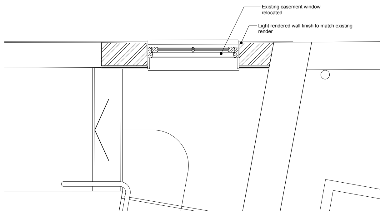
Proposed Window Plan Detail
