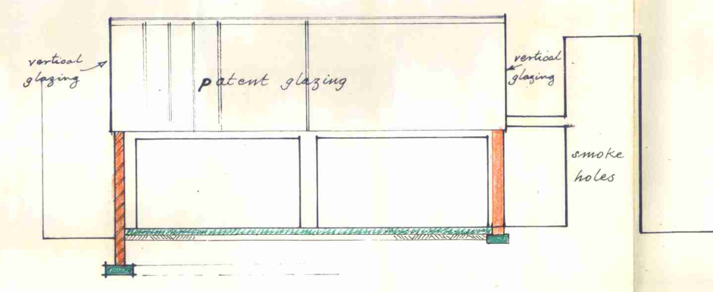
SECTION B-B
