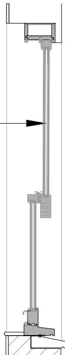
3 TYPE 66 C SECTION
