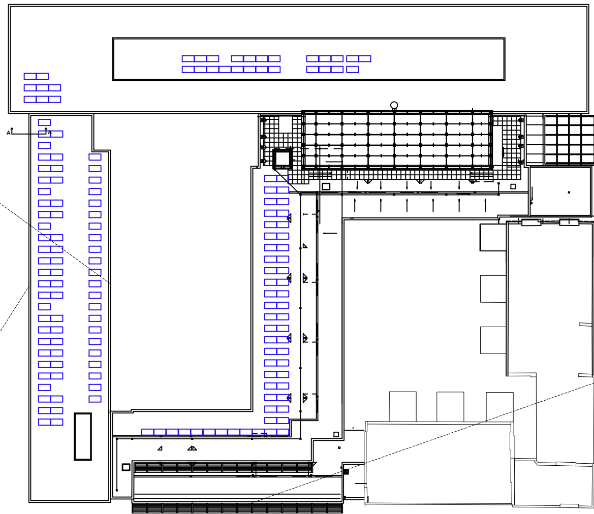
Proposed Roof Plan 1:500
