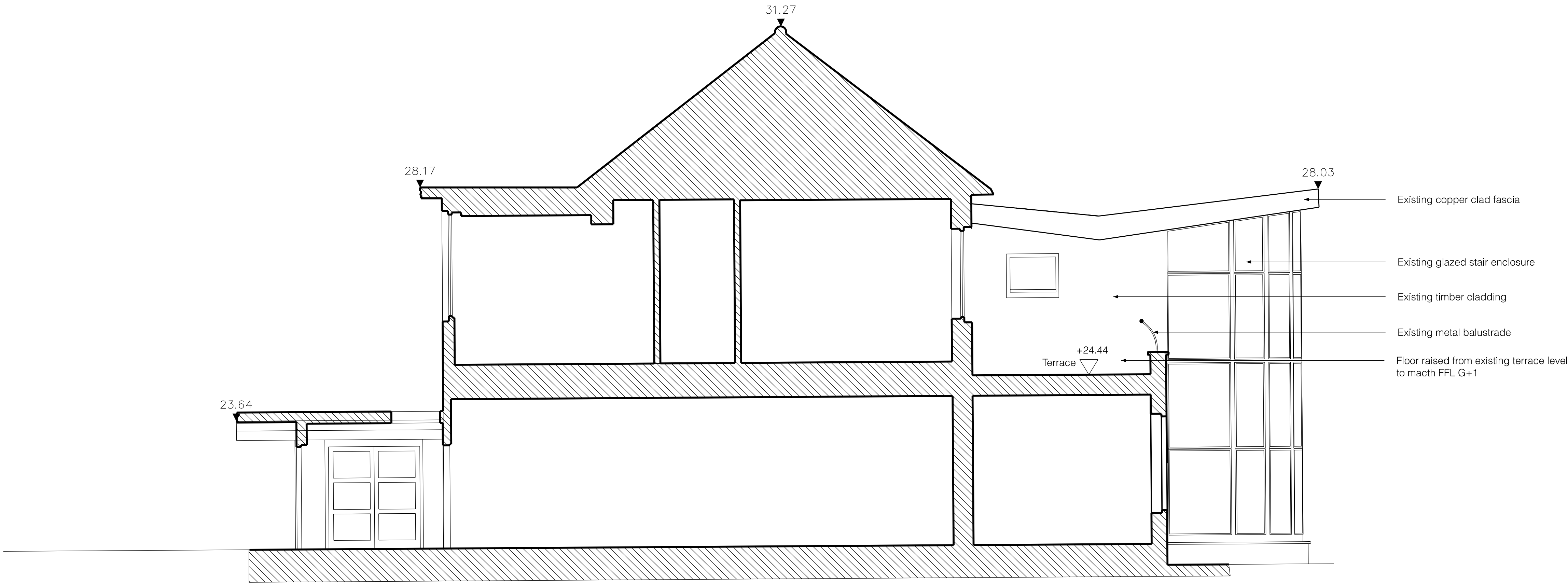
1 Existing Section AA 1:50 @ A1
