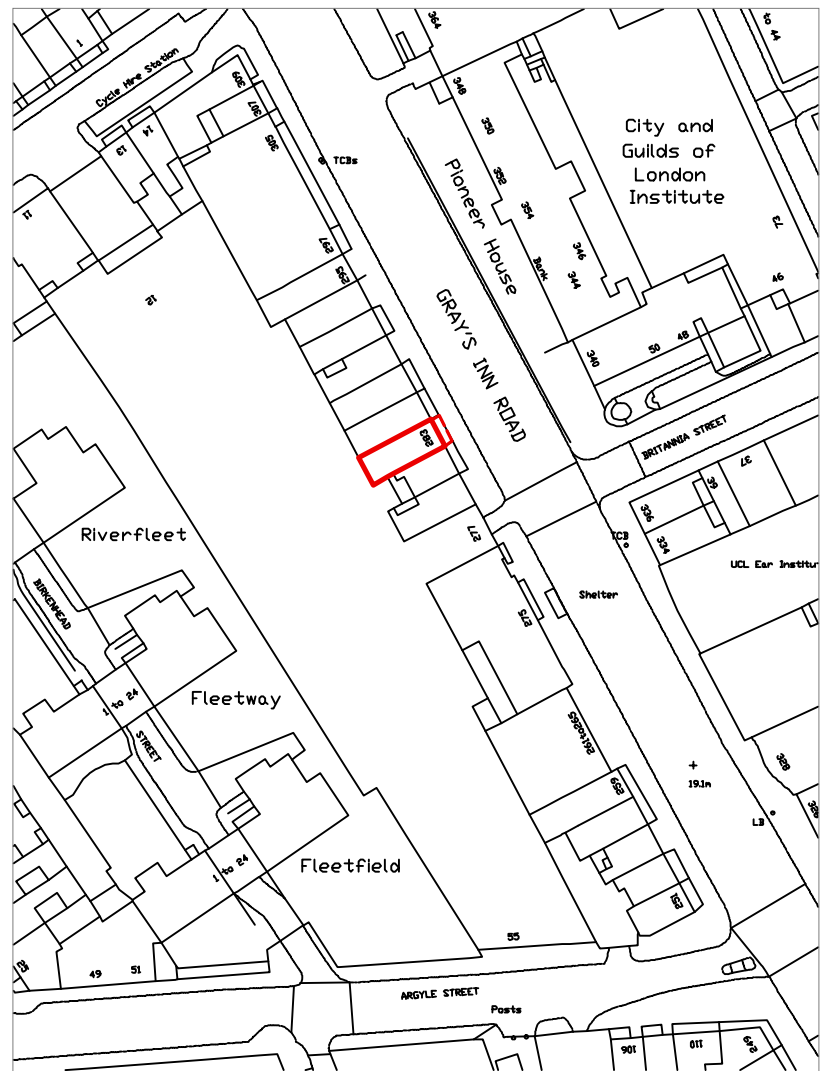
LOCATION PLAN AT 1:1250 SCALE & NORTH UP ^
