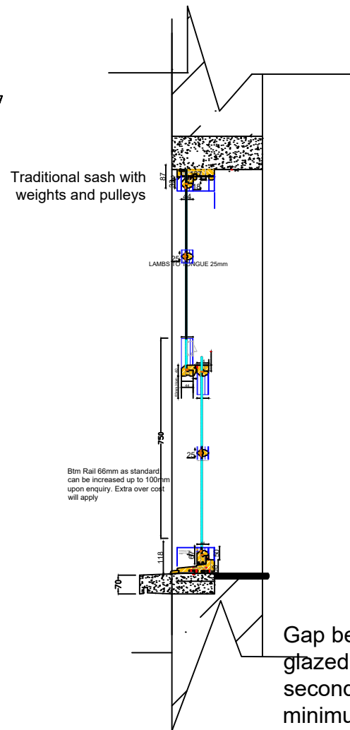
Window Section A-A
