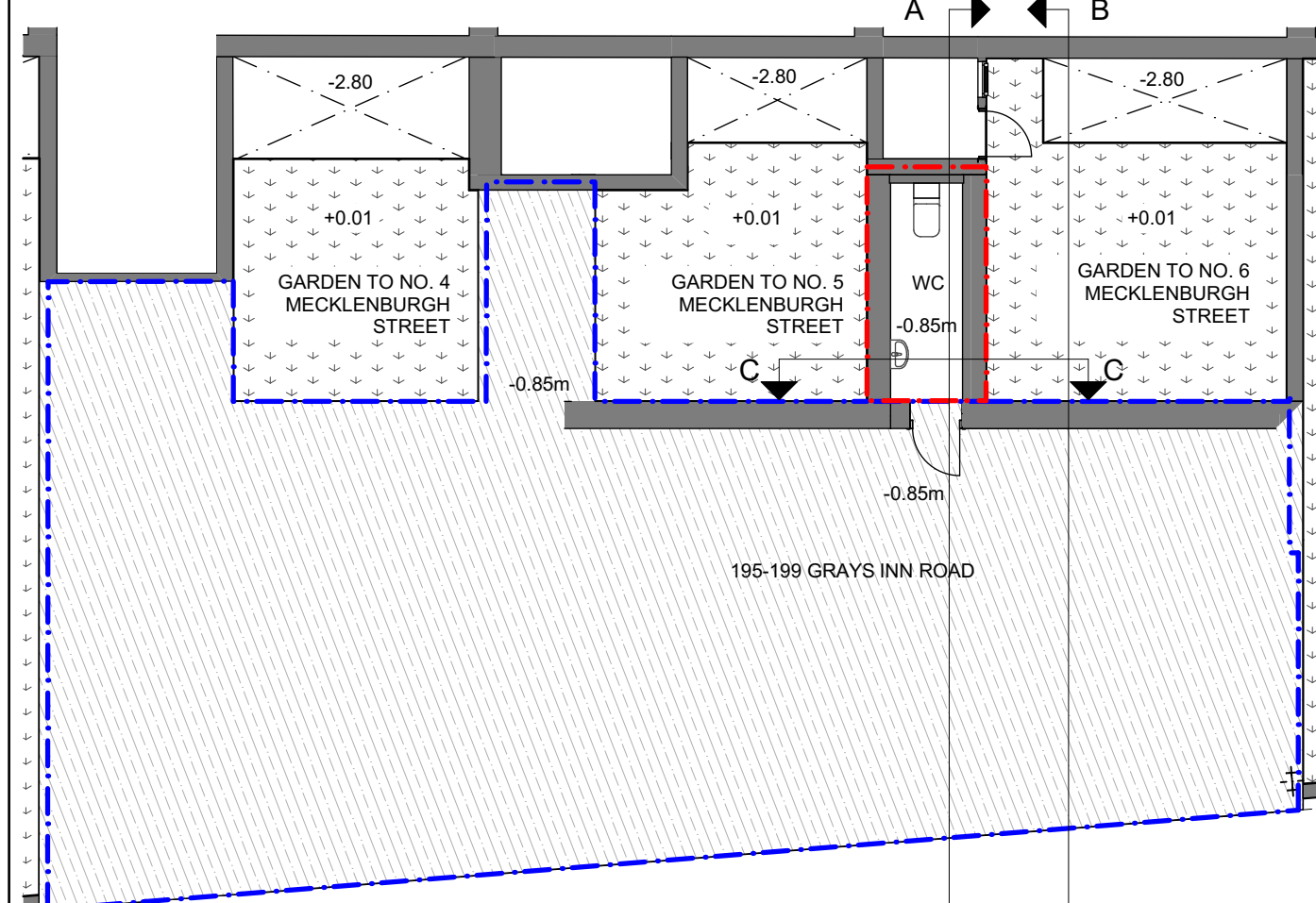
PROPOSED LOWER GROUND FLOOR
