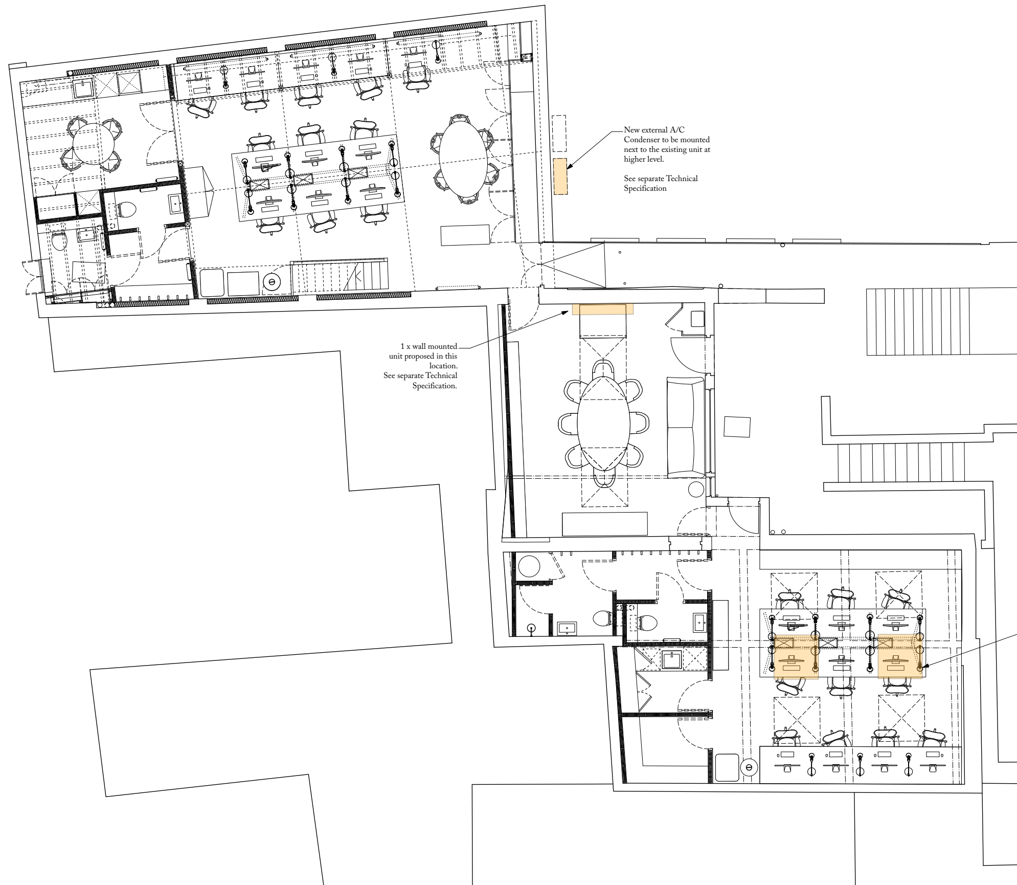
1 PROPOSED GROUND FLOOR PLAN WITH AC LAYOUT 1:100@A3
