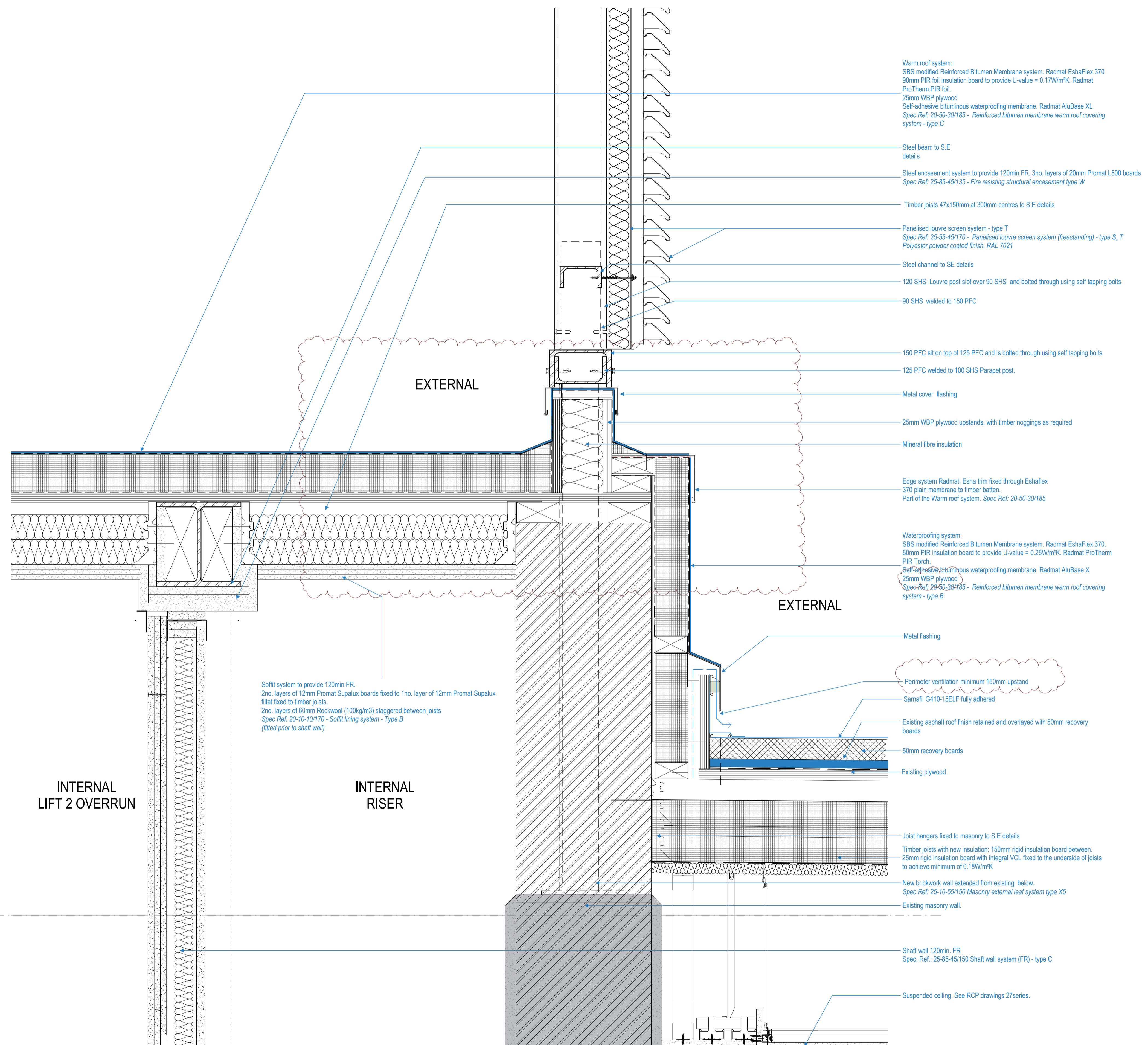
A 5112 Lift 2 Overrun - Section A 1 : 5
