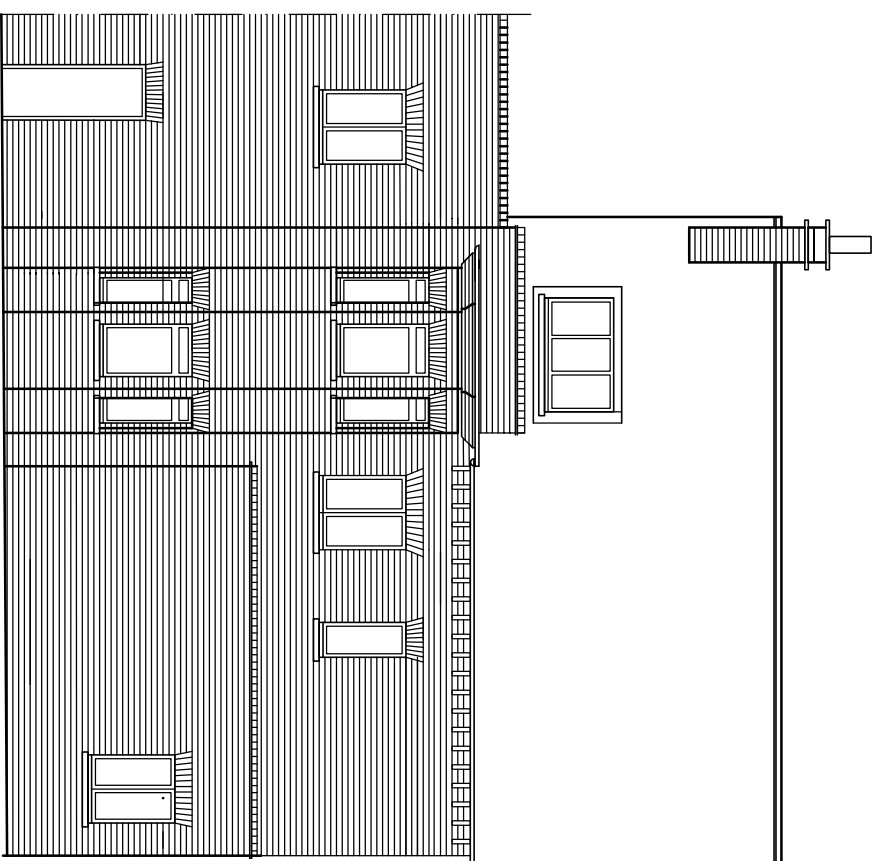
REAR ELEVATION
