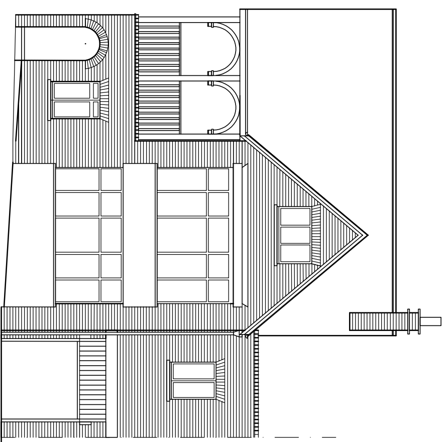
FRONT ELEVATION ON TO ROSSLYN HILL
