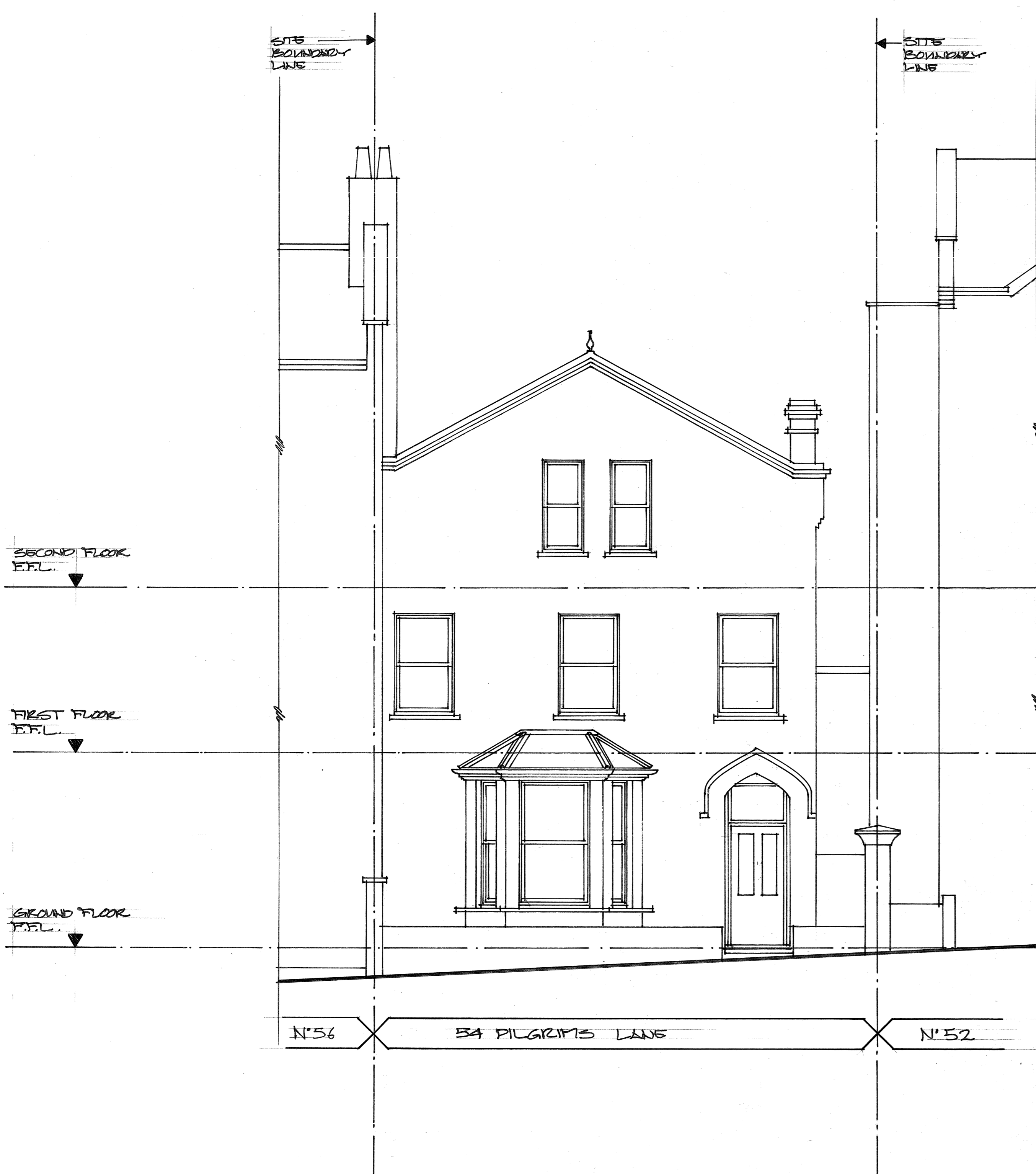
EXISTING FRONT ELEVATION
