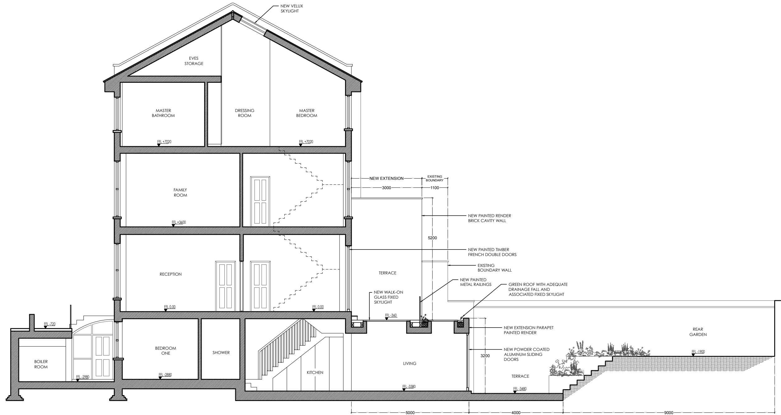
PROPOSED SECTION A - A' SCALE 1:100
