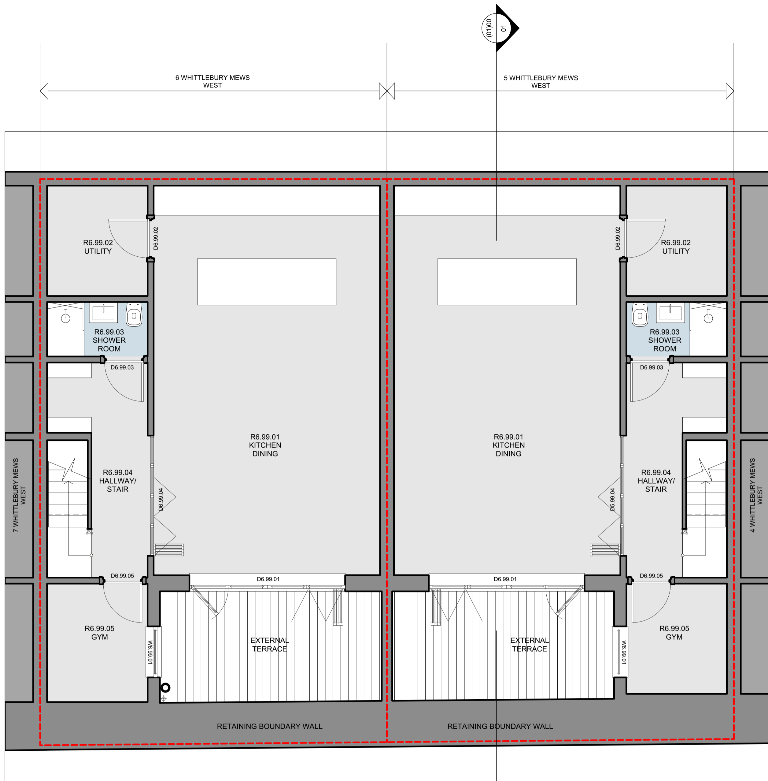
1 PROPOSED B01 PLAN Scale: 1:50
