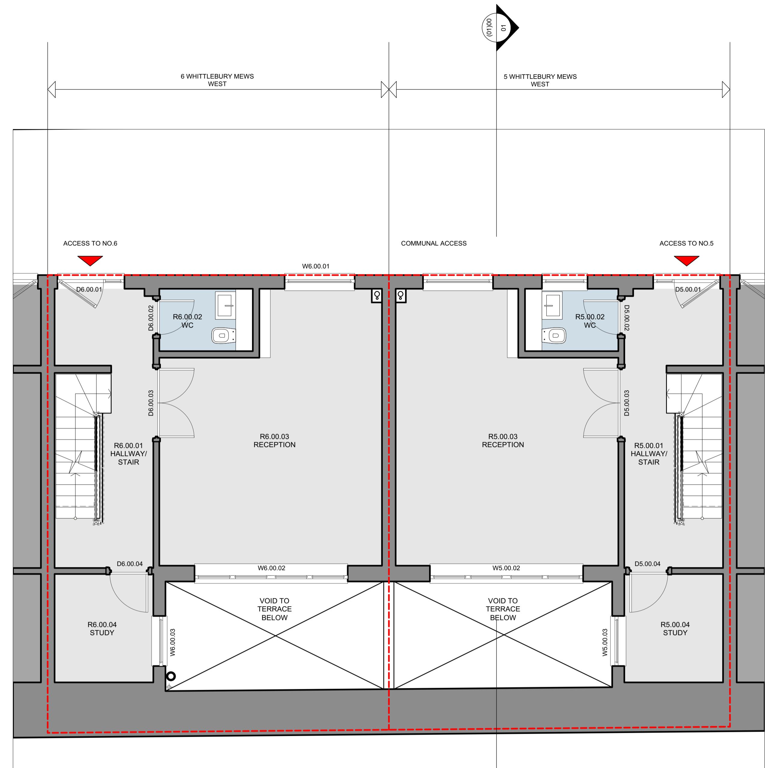
2 PROPOSED L01 PLAN Scale: 1:50
