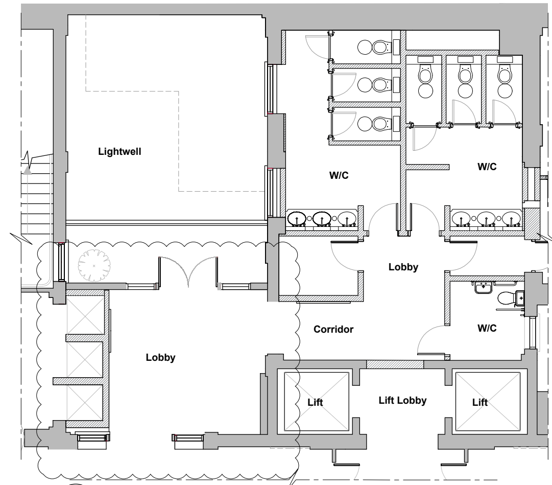
03 LIGHTWELL EXTENSION - GROUND FLOOR PLAN AS PROPOSED 7811 1:100 @ A3
