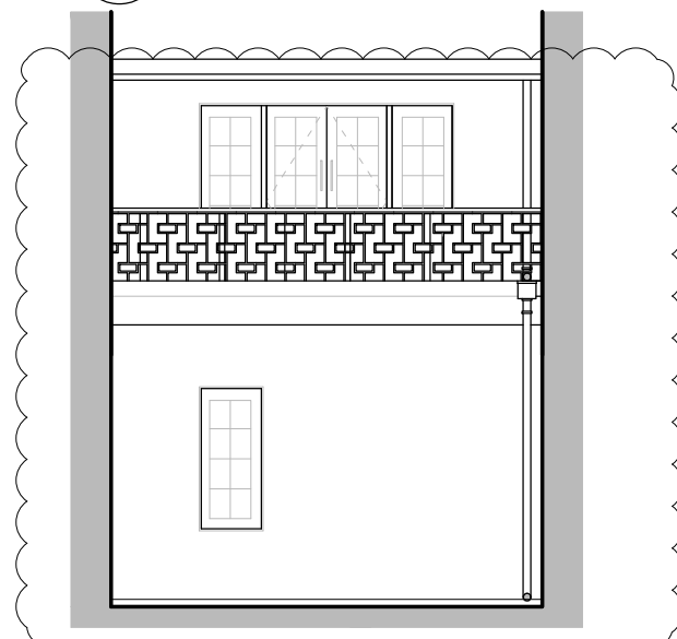
02 LIGHTWELL EXTENSION - SECTION AS PROPOSED 7811 1:100 @ A3
