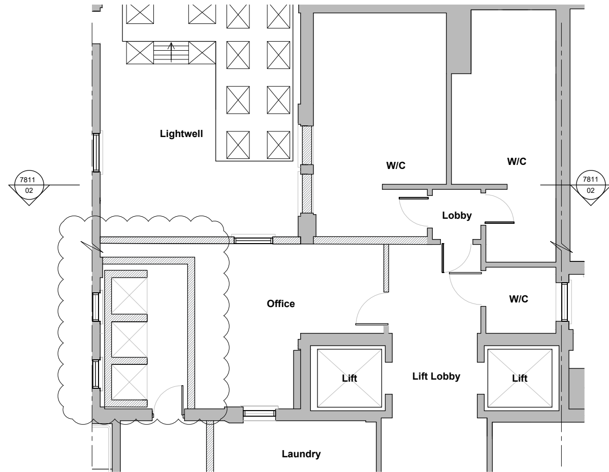
01 LIGHTWELL EXTENSION - BASEMENT PLAN AS PROPOSED 7811 1:100 @ A3
