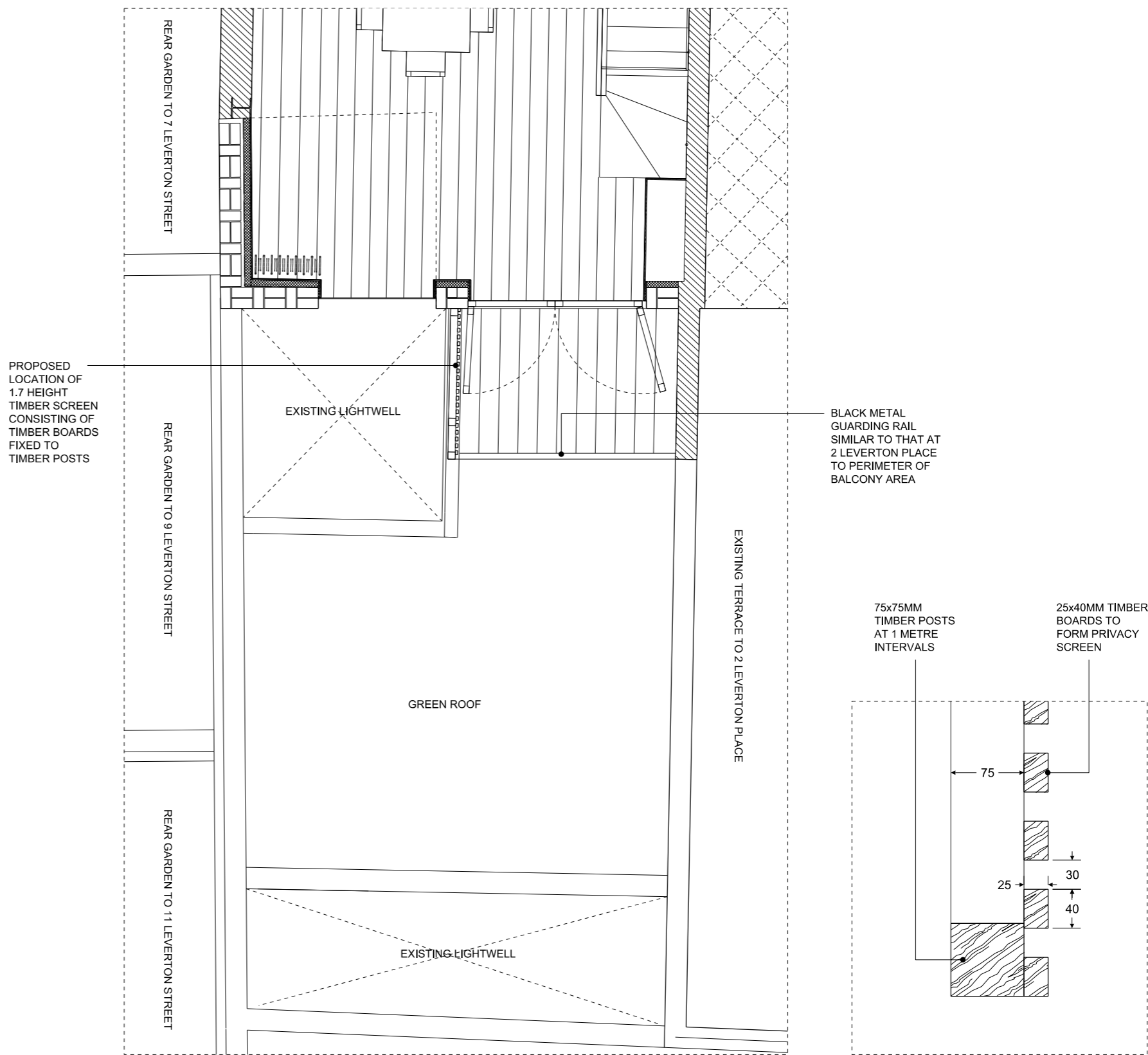
02 PROPOSED FIRST FLOOR SCREEN LOCATION PLAN 02-700 1:50 @ A3
